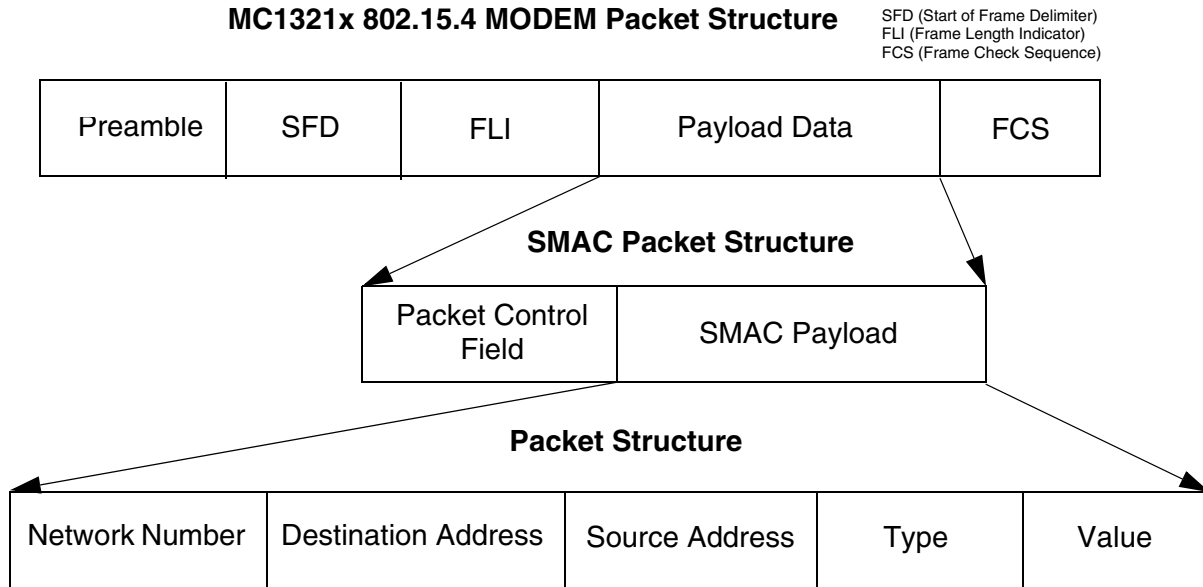
Figure 10. Packet Structure
