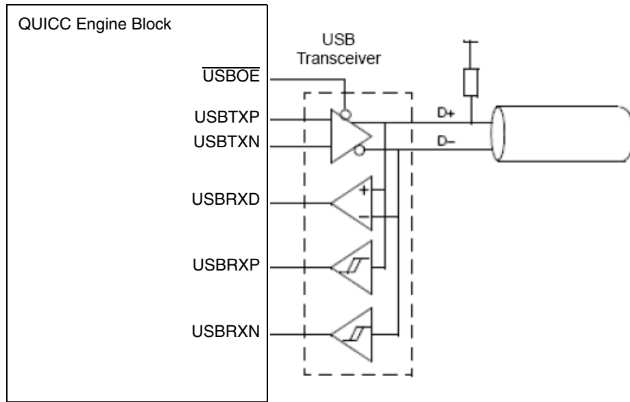
Figure 4. USB Interface
