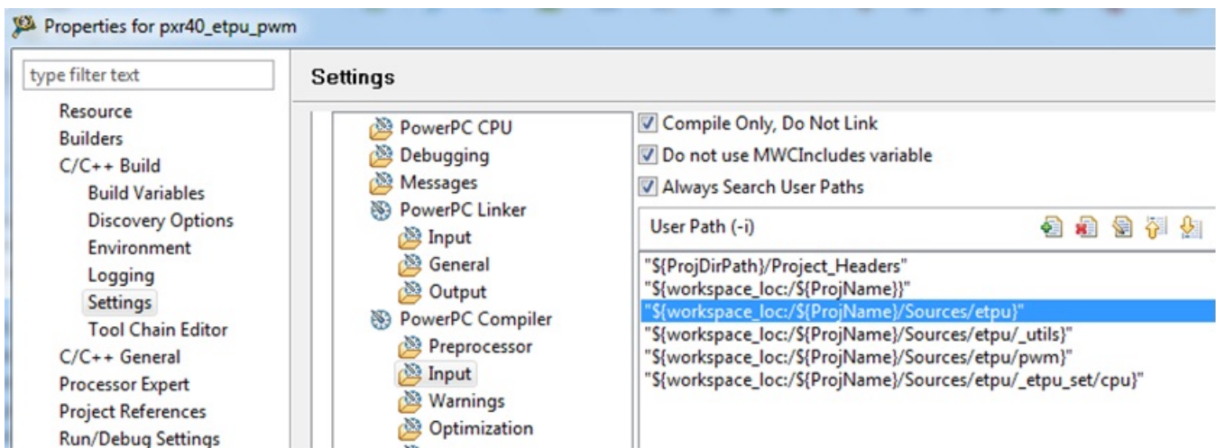
Figure 1. Include directories
