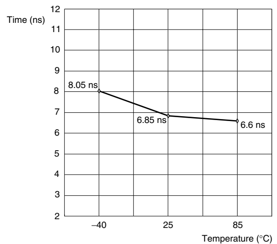
Fig 26. Maximum allowable time for V_{DD} = 0 V and data in registers is retained
