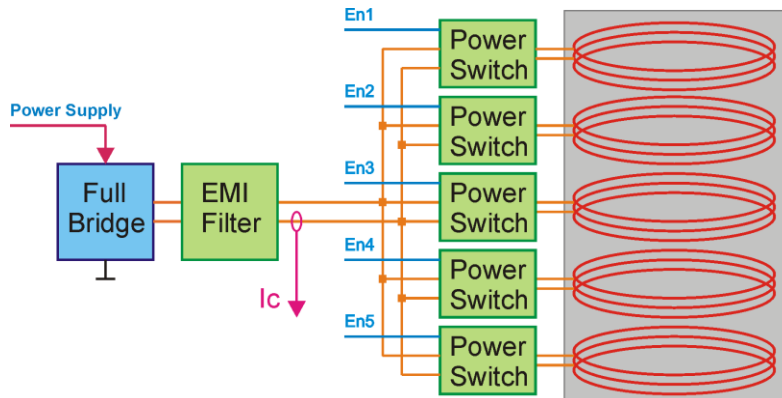
Figure 5 Power multiplexer
