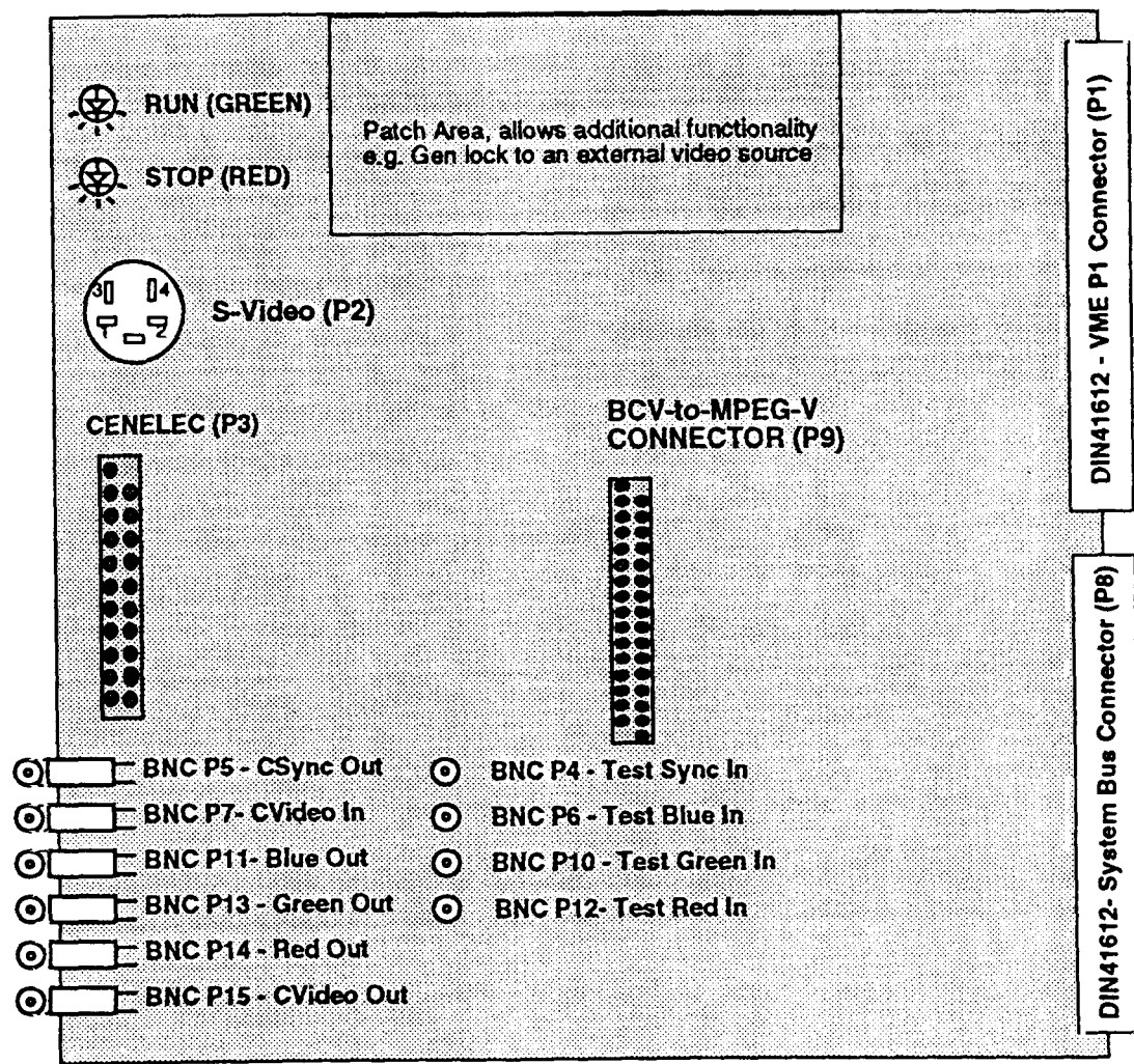
Figure 5. Layout of BCV connectors
