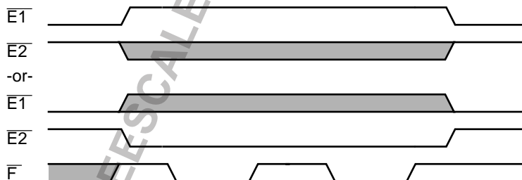
Figure 1-1 Pseudo Static RAM Auto Refresh Timing in which 2 rows are refreshed in succession. Note that either \bar{E1} or \bar{E2} can disable the device. Please refer to the data sheets specific to the PSRAMs selected for any particular application.
