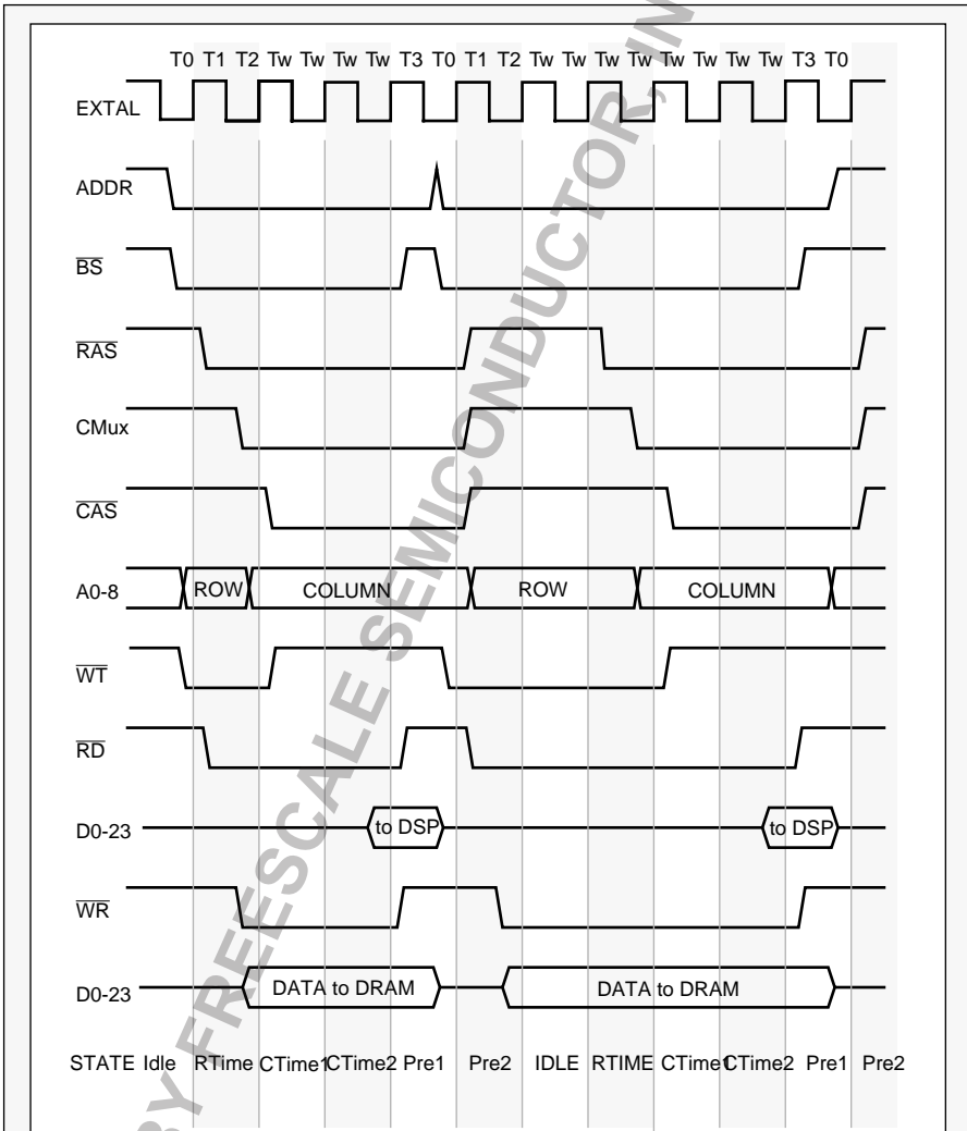
Figure 2-3 DSP56001-to-DRAM Timing shows two back to back write operations.
