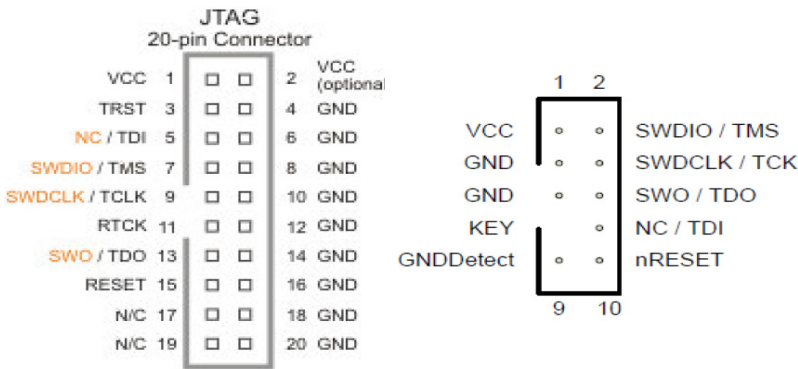
Figure 14. Debug headers
