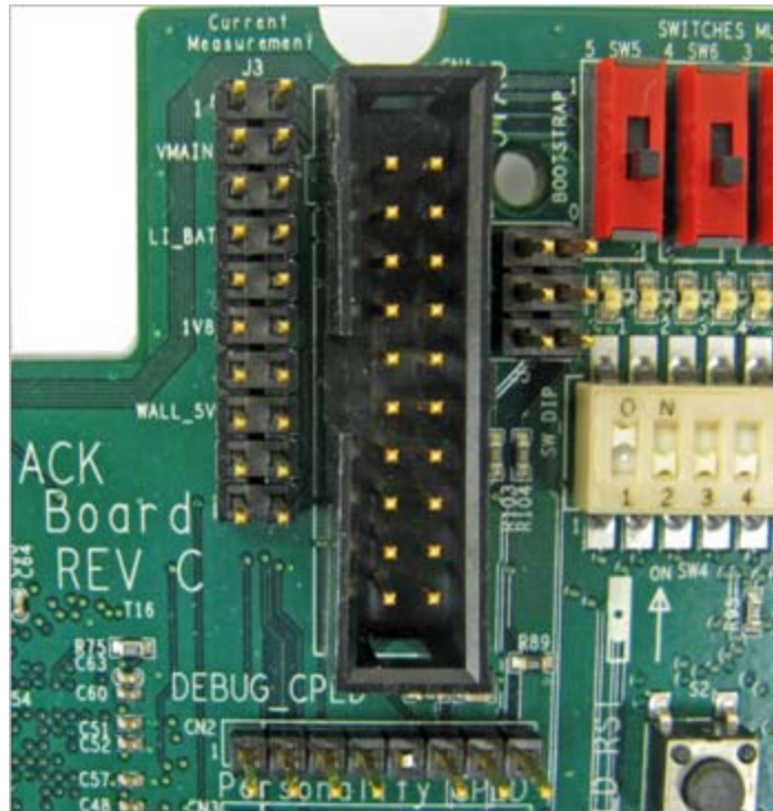
Figure 3 Current Measurement Connector Detail
