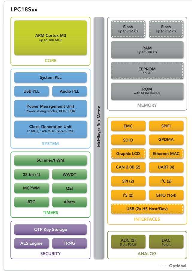
LPC18Sxx block diagram
