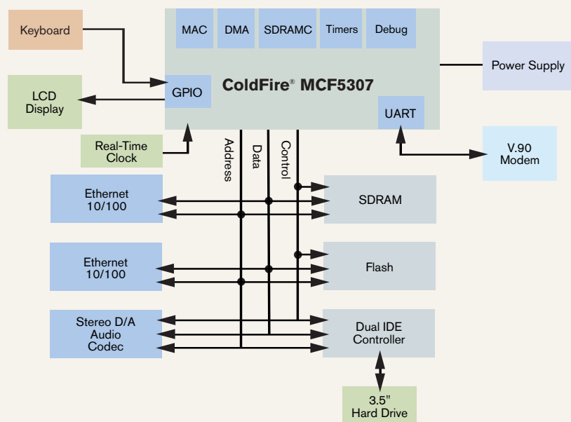
MCF5307 BLOCK DIAGRAM
