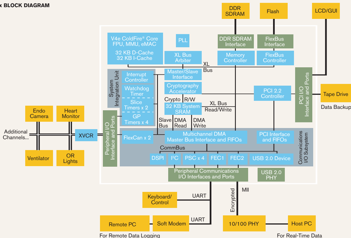
MCF548x BLOCK DIAGRAM
