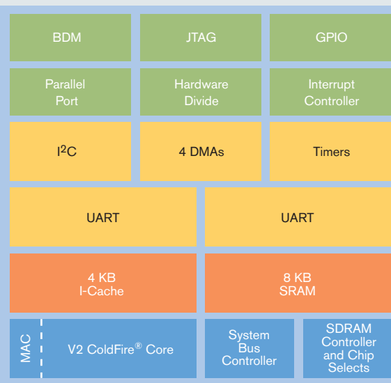
MCF5206e BLOCK DIAGRAM
