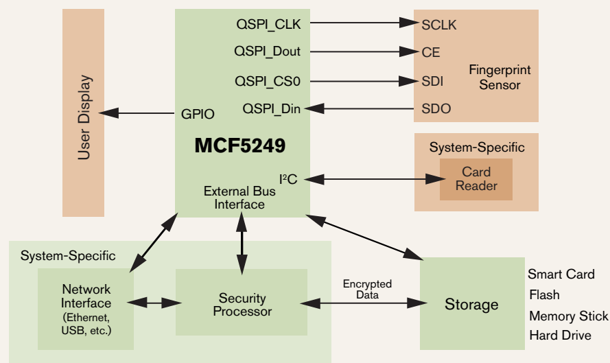
MCF5249 BLOCK DIAGRAM
