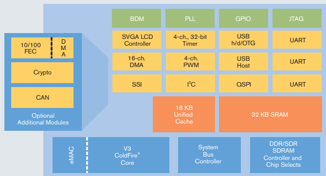
MCF532x BLOCK DIAGRAM
