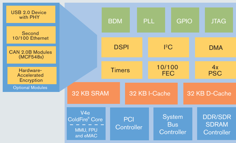
MCF547x AND MCF548x BLOCK DIAGRAM
