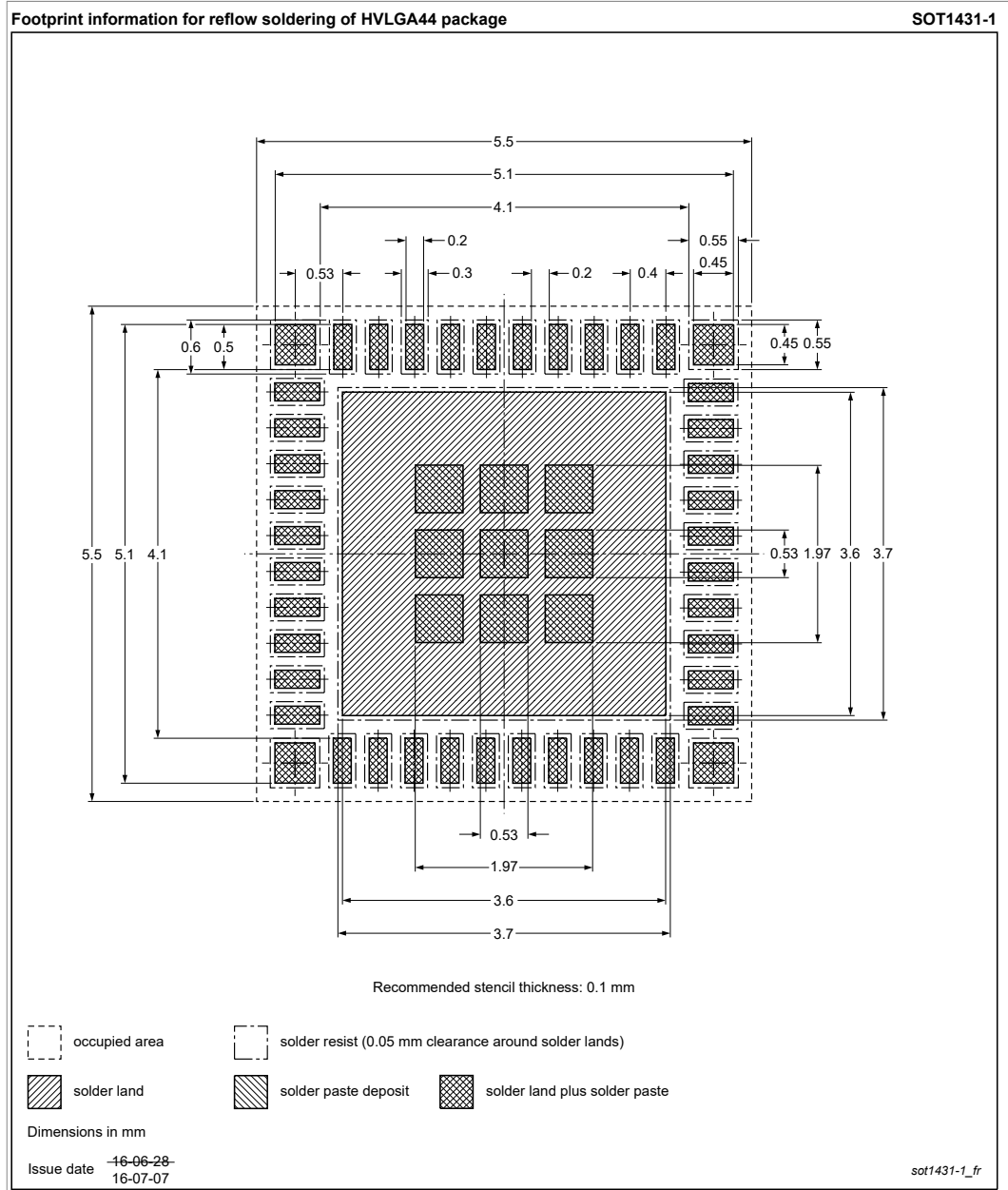
Figure 54. Footprint information
