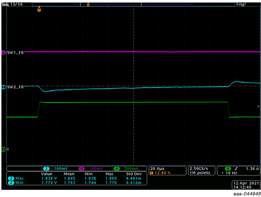
Figure 23. SW2 Load Transient Response
