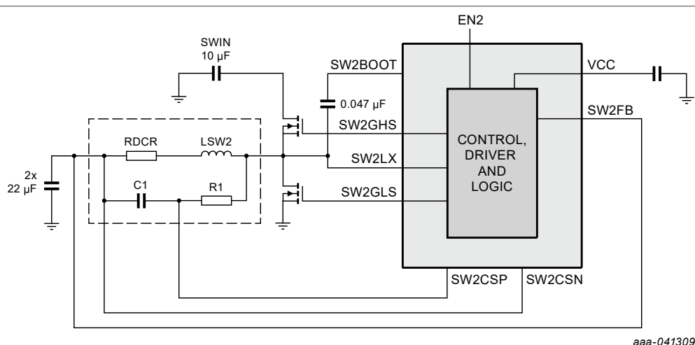
Figure 11. DCR current sense with a single capacitor
