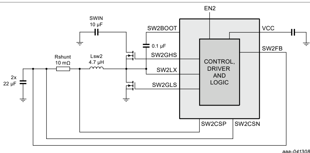
Figure 10. SW2 application schematic with Rshunt current sensing
