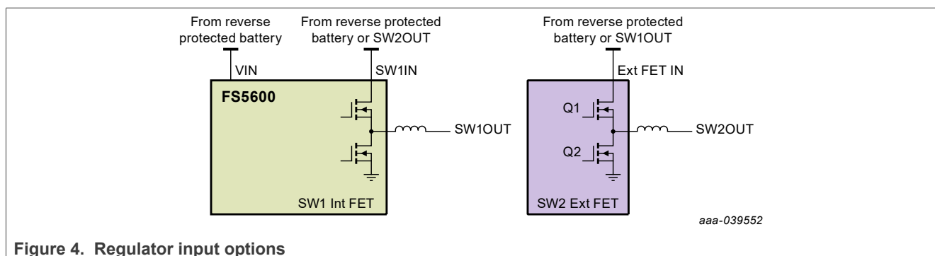
Figure 4. Regulator input options
