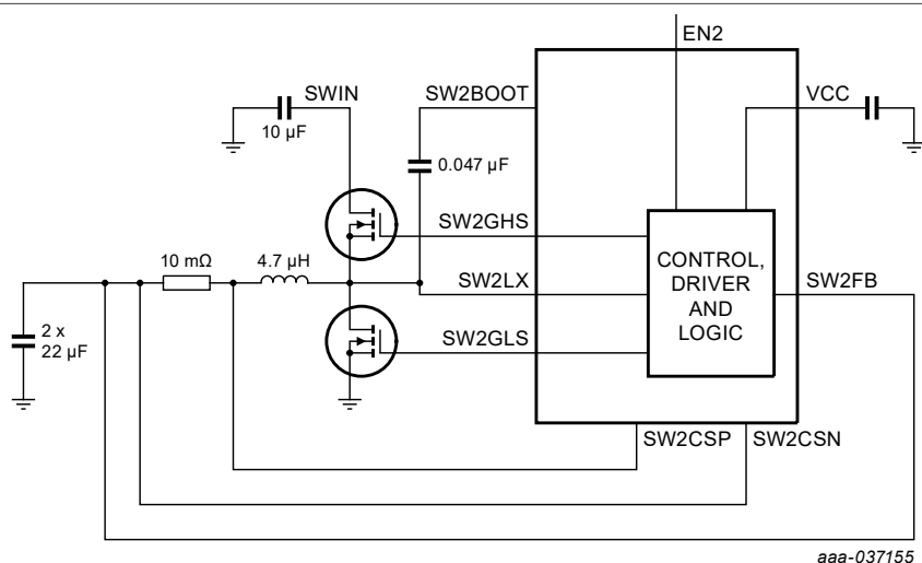
Figure 9. SW2 high-level block diagram
