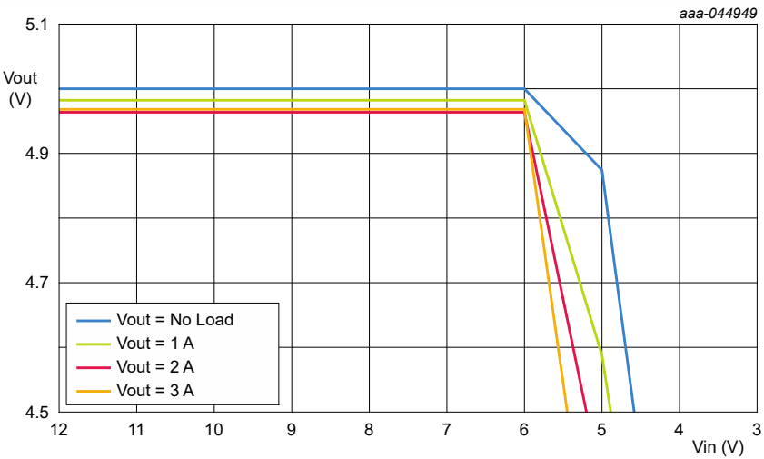
Figure 24. SW1 Dropout Performance
