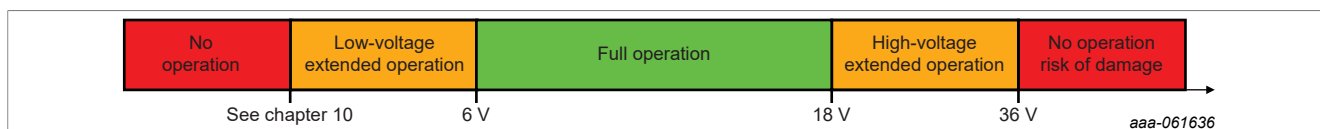
Figure 3. Input operation range
