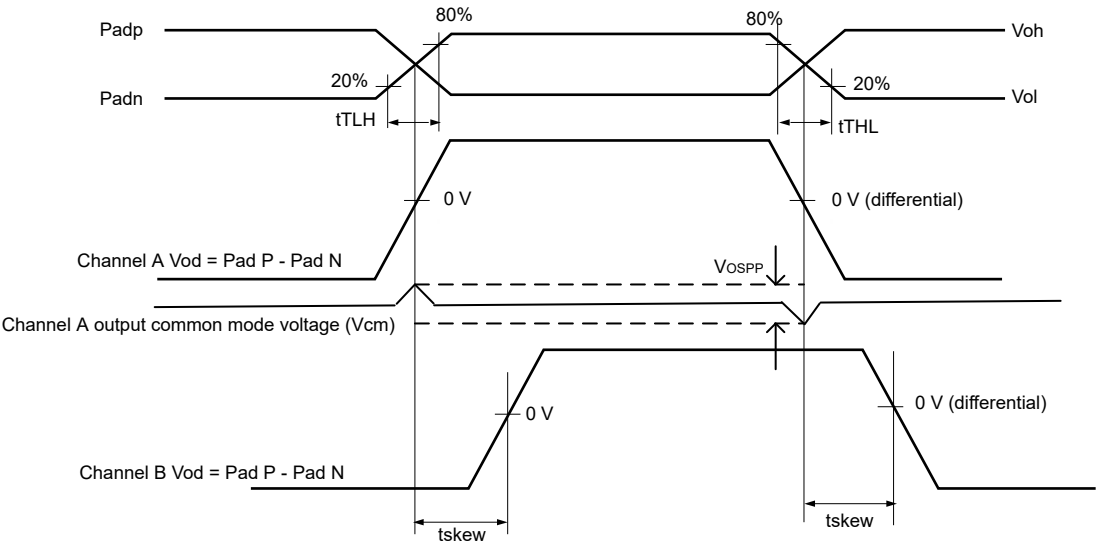
Figure 7. Output transition time waveform
