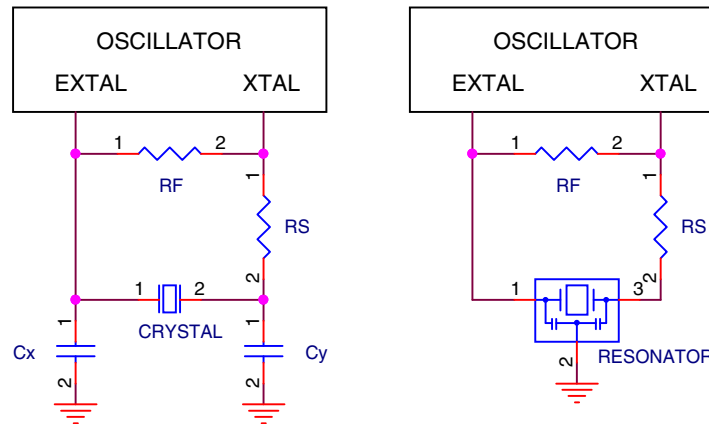
Figure 36. Crystal connection – Diagram 3
