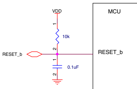
Figure 31. Reset circuit
