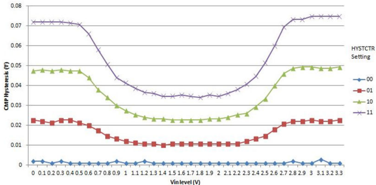
Figure 20. Typical hysteresis vs. Vin level (VDD = 3.3 V, PMODE = 1)
