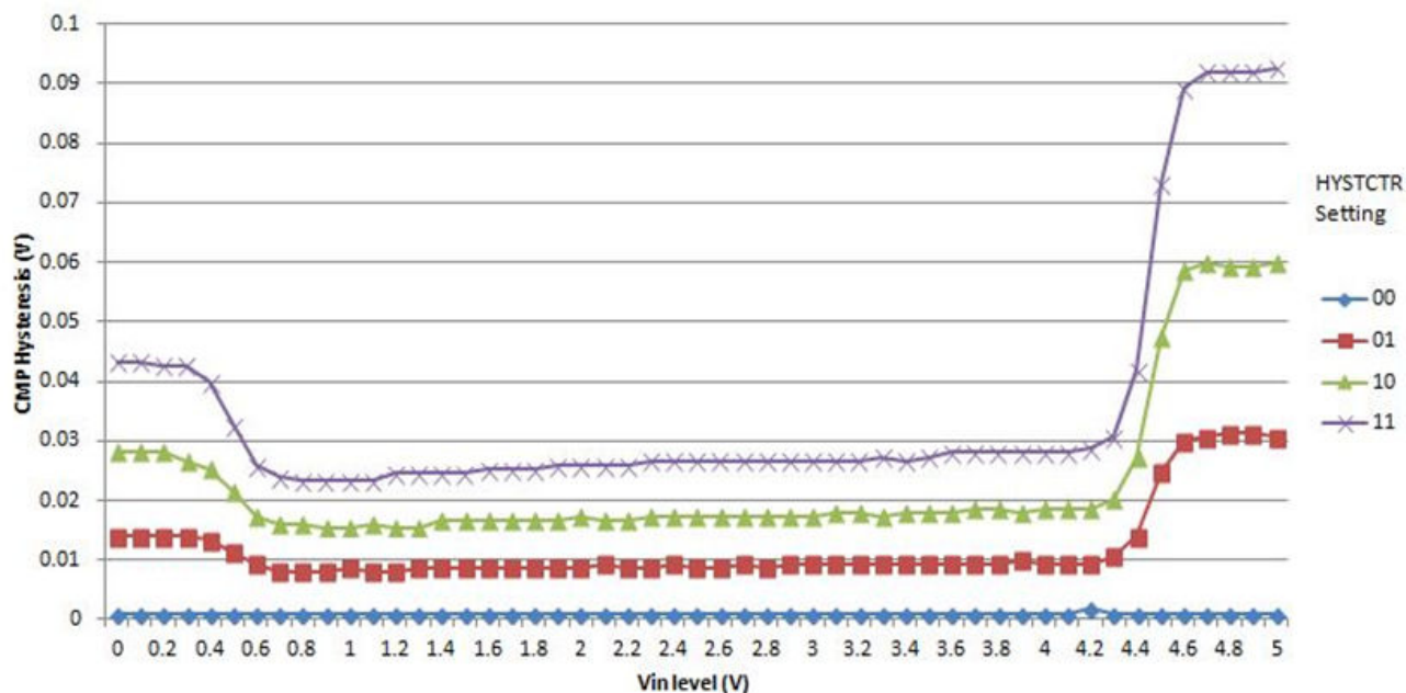
Figure 22. Typical hysteresis vs. Vin level (VDD = 5 V, PMODE = 1)
