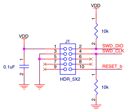
Figure 34. SWD debug interface
