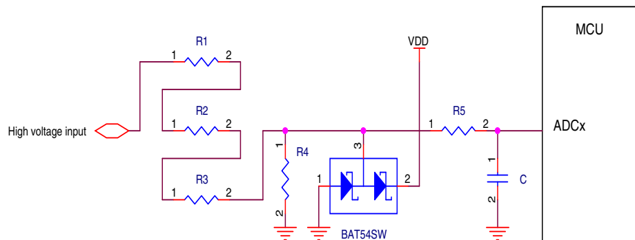
Figure 30. High voltage measurement with an ADC input
