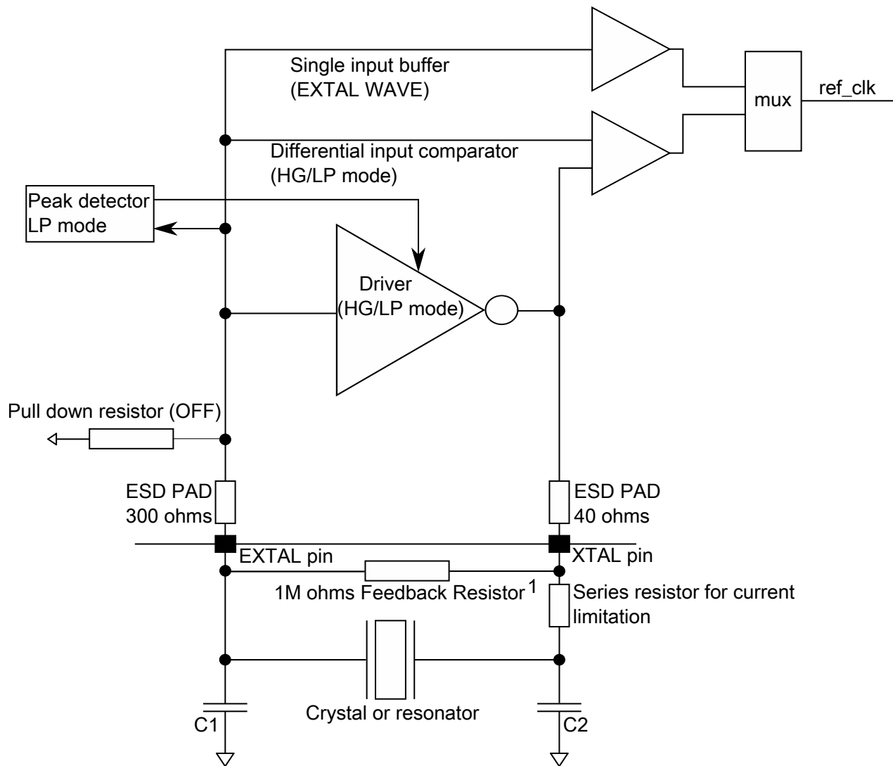
Figure 17. Oscillator connections scheme (OSC)
