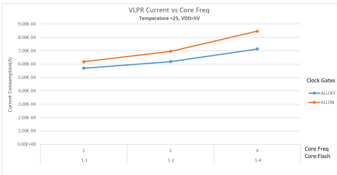
Figure 15. VLPR mode supply current vs. core frequency
