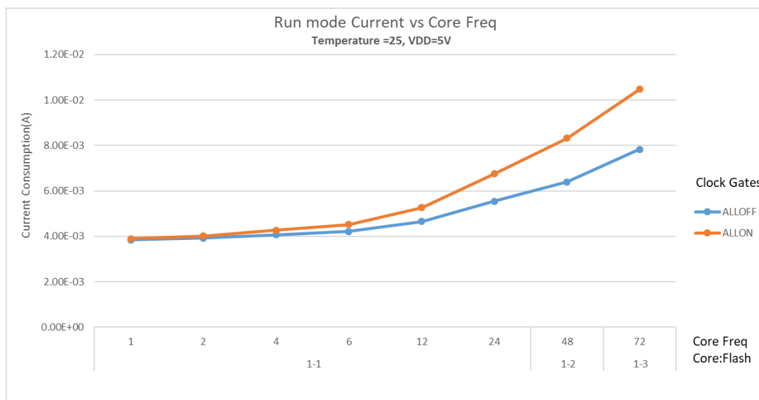
Figure 14. Run mode supply current vs. core frequency
