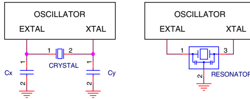
Figure 35. Crystal connection – Diagram 2
