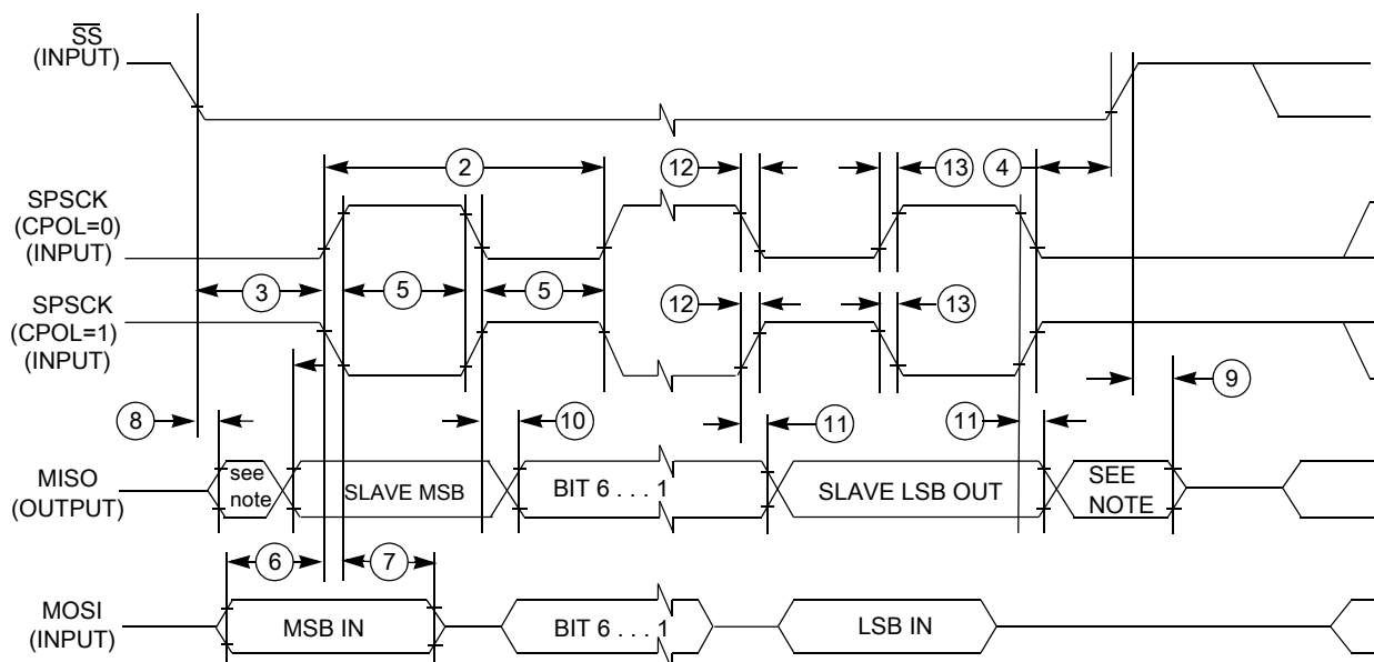
Figure 25. LPSPI slave mode timing (CPHA = 0)
