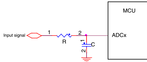
Figure 29. RC circuit for ADC input
