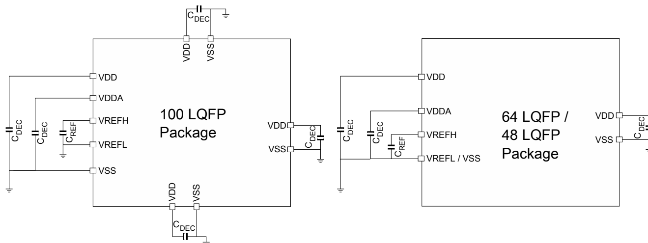
Figure 13. Pinout decoupling
