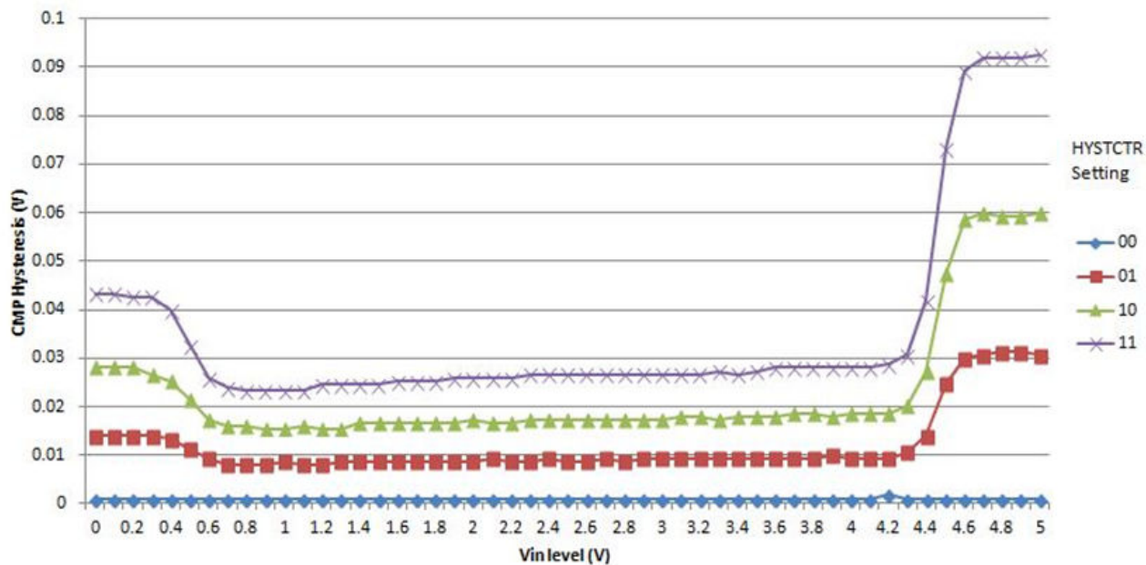
Figure 21. Typical hysteresis vs. Vin level (VDD = 5 V, PMODE = 0)
