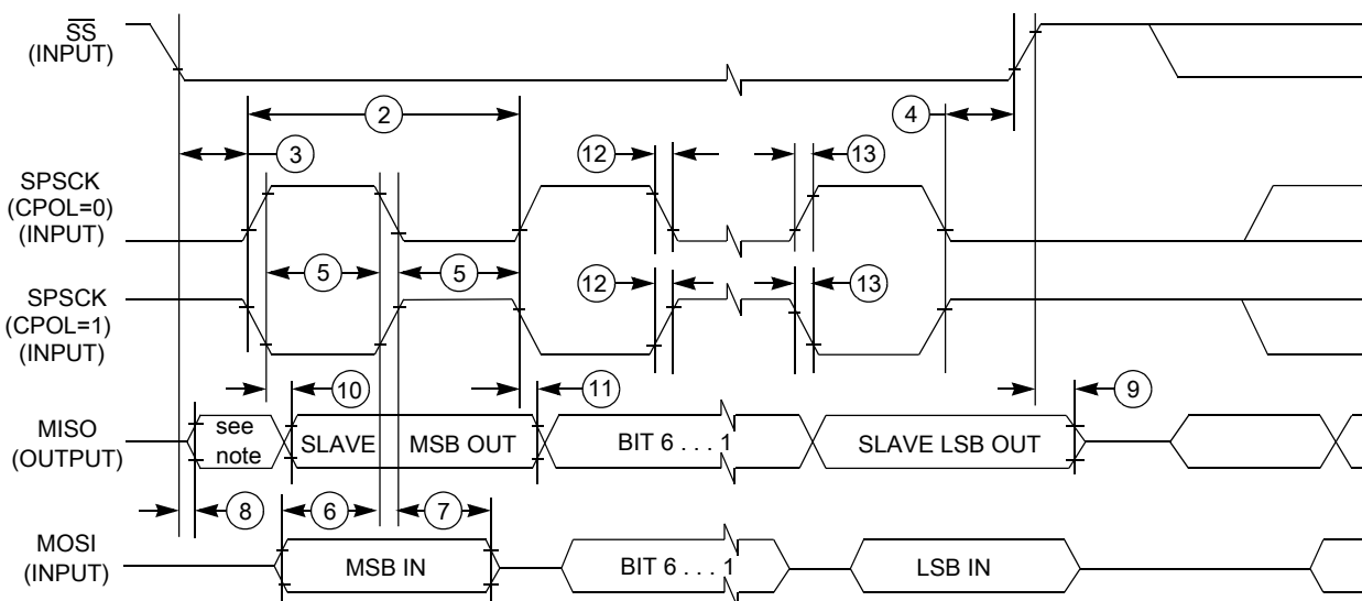
Figure 26. LPSPI slave mode timing (CPHA = 1)
