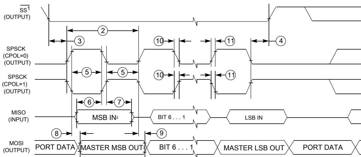
Figure 24. LPSPI master mode timing (CPHA = 1)
