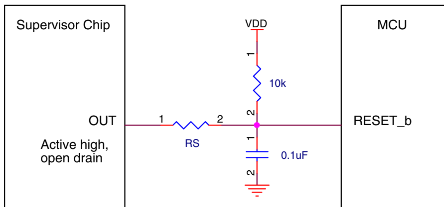
Figure 32. Reset signal connection to external reset chip
