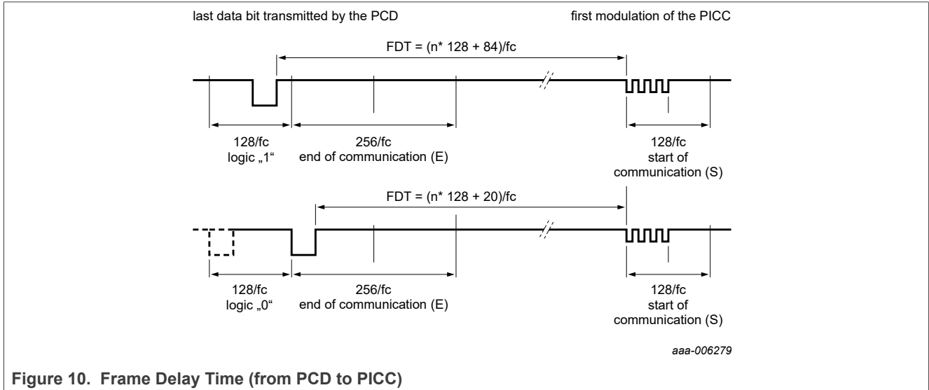
Figure 10. Frame Delay Time (from PCD to PICC) Remark: Due to the coding of commands, the measured timings usually exclude (a part of) the end of communication. Consider this factor when comparing the specified with the measured times.
