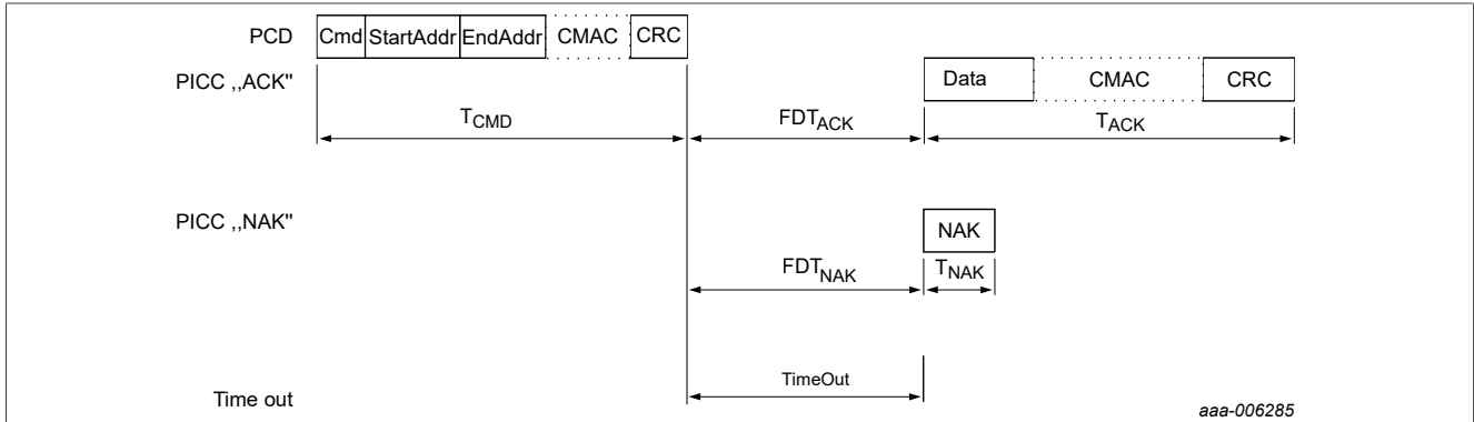
Figure 13. FAST_READ command
