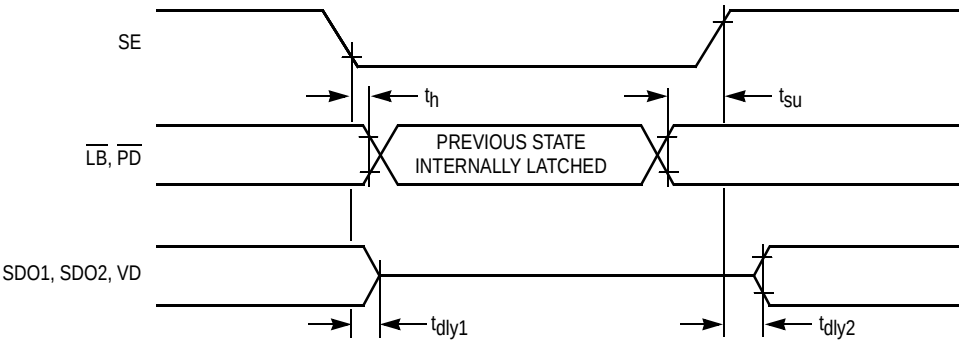
Figure 6. SE Pin Timing
