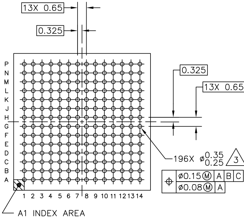
BOTTOM VIEW
