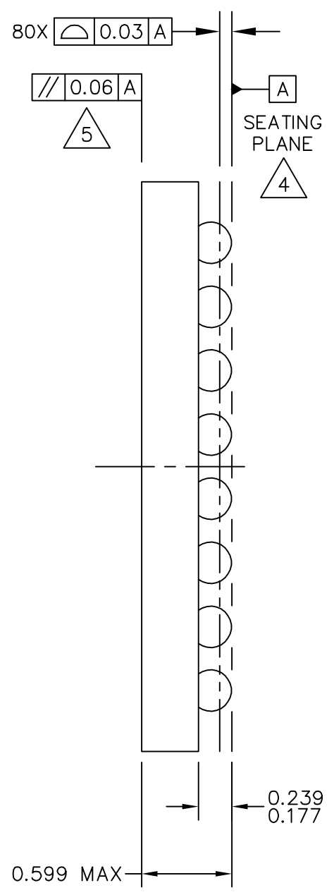
VIEW D-D
