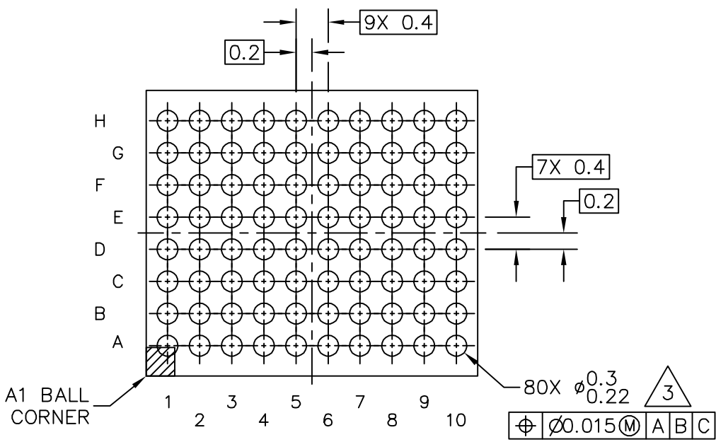
BOTTOM VIEW
