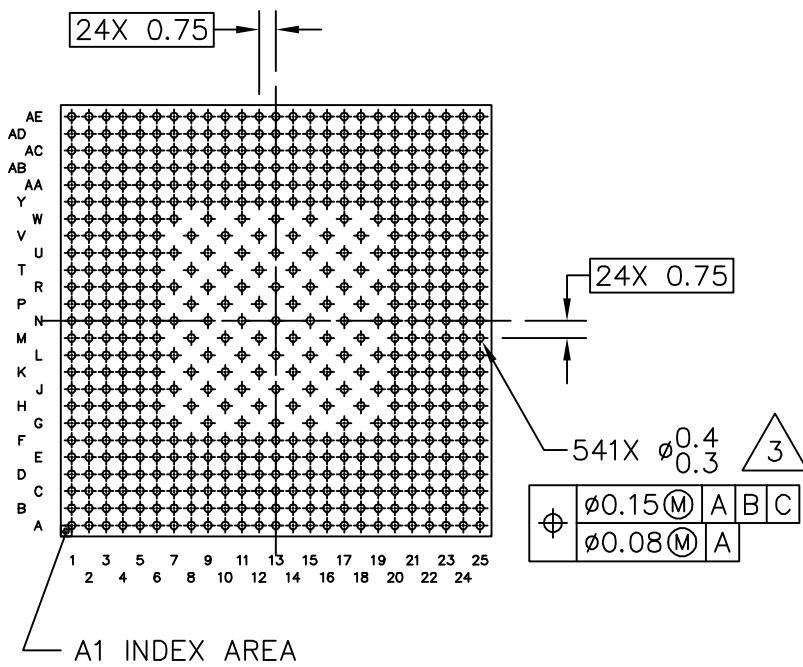
BOTTOM VIEW
