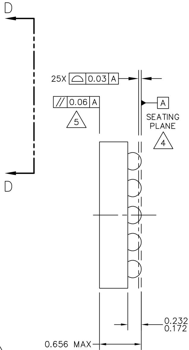
VIEW D-D
