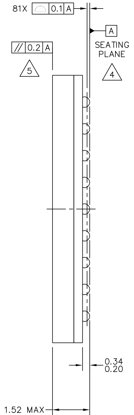
SIDE VIEW
