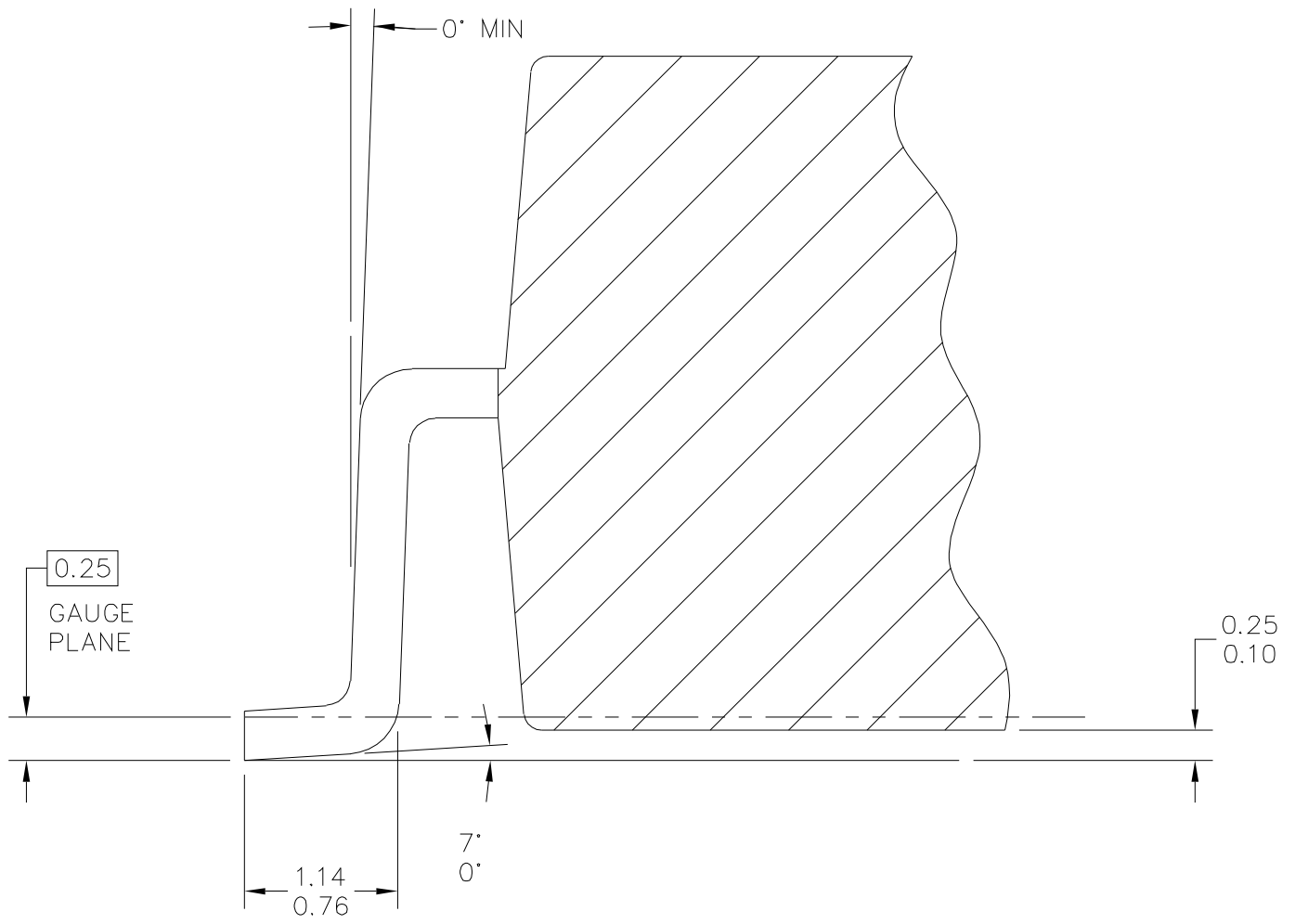
SECTION B-B
