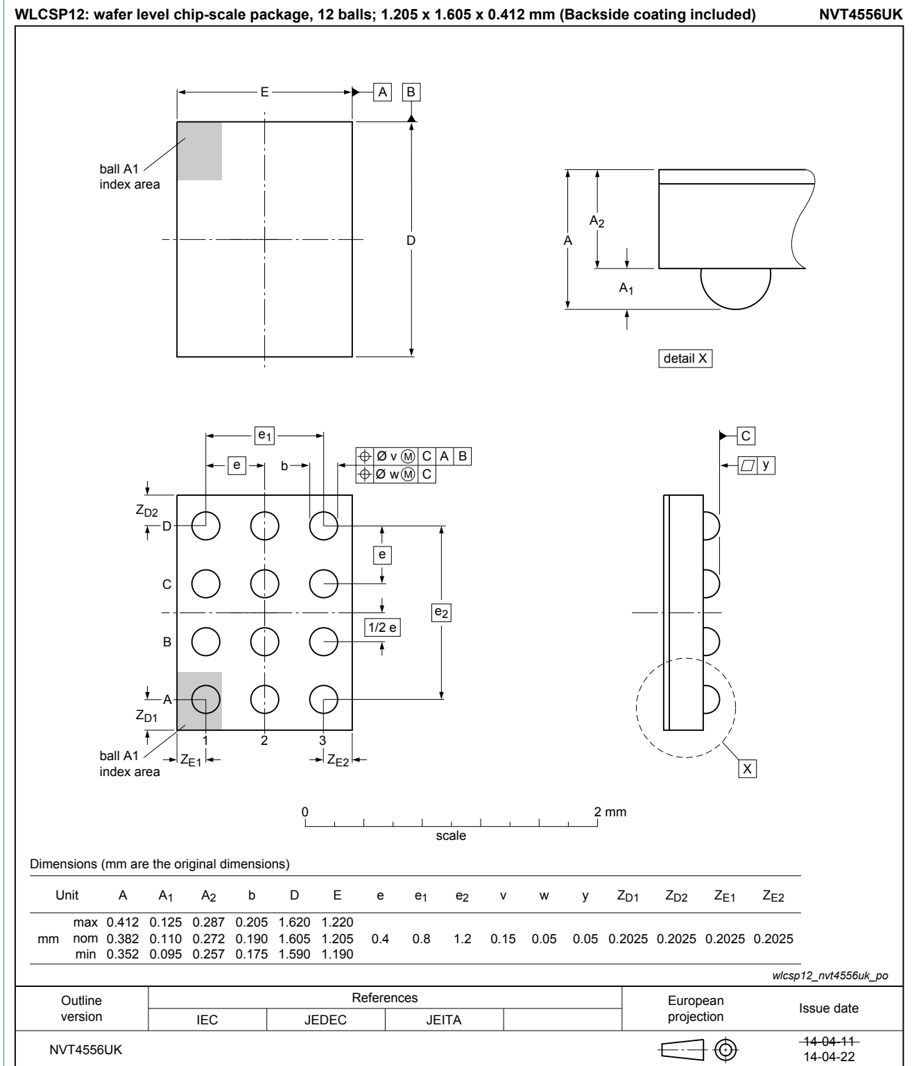
Figure 1. Package outline WLCSP12 NVT4556UK
