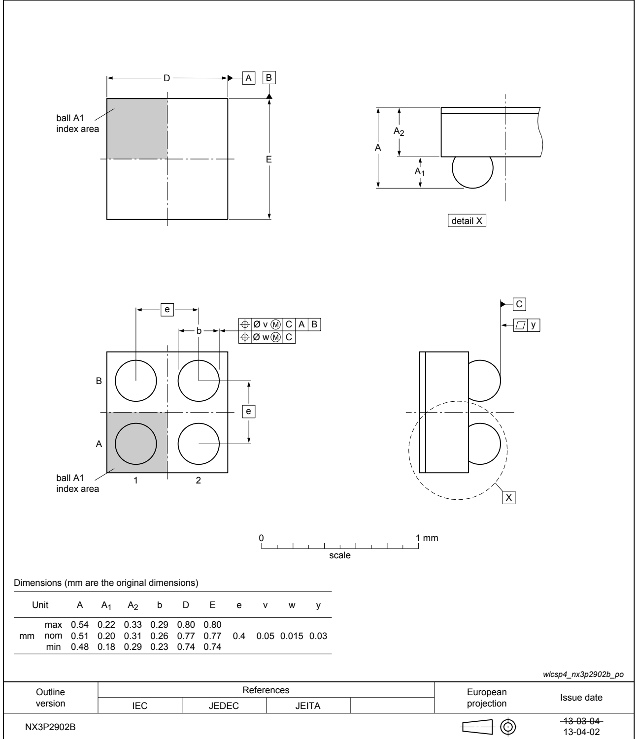
Fig. 1. Package outline WLCSP (OL-NX3P2902B)
