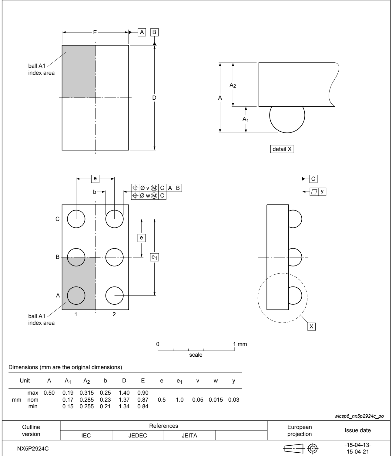
Fig. 1. Package outline WLCSP6 (OL-NX5P2924C)
