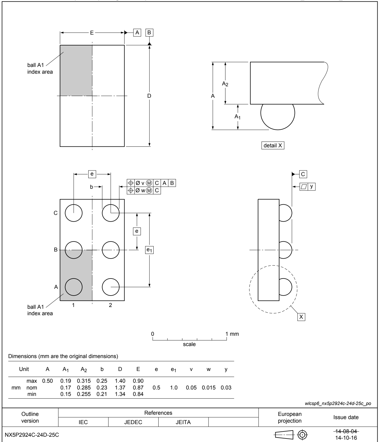
Fig. 1. Package outline WLCSP6 (OL-NX5P2924C_NX5P2924D_NX5P2925C)
