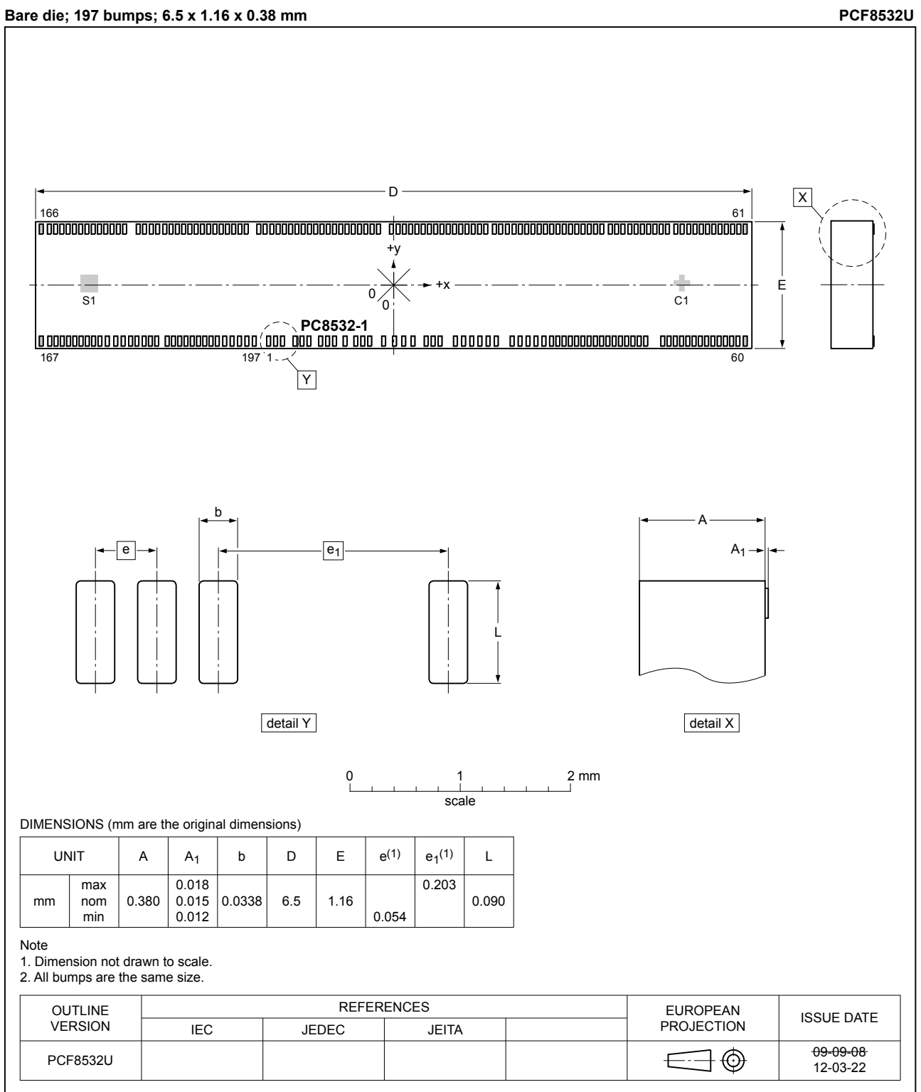
Fig. 1. Package outline UC (OL-PCF8532U)
