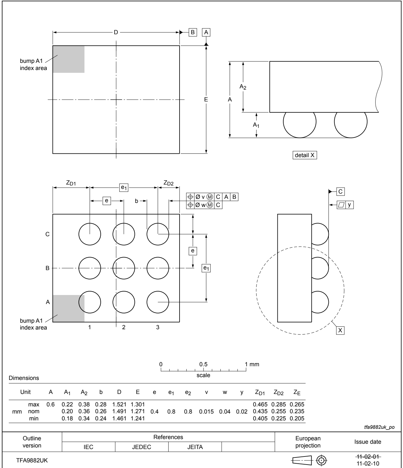
Fig. 1. Package outline WLCSP (OL-TFA9882UK)
