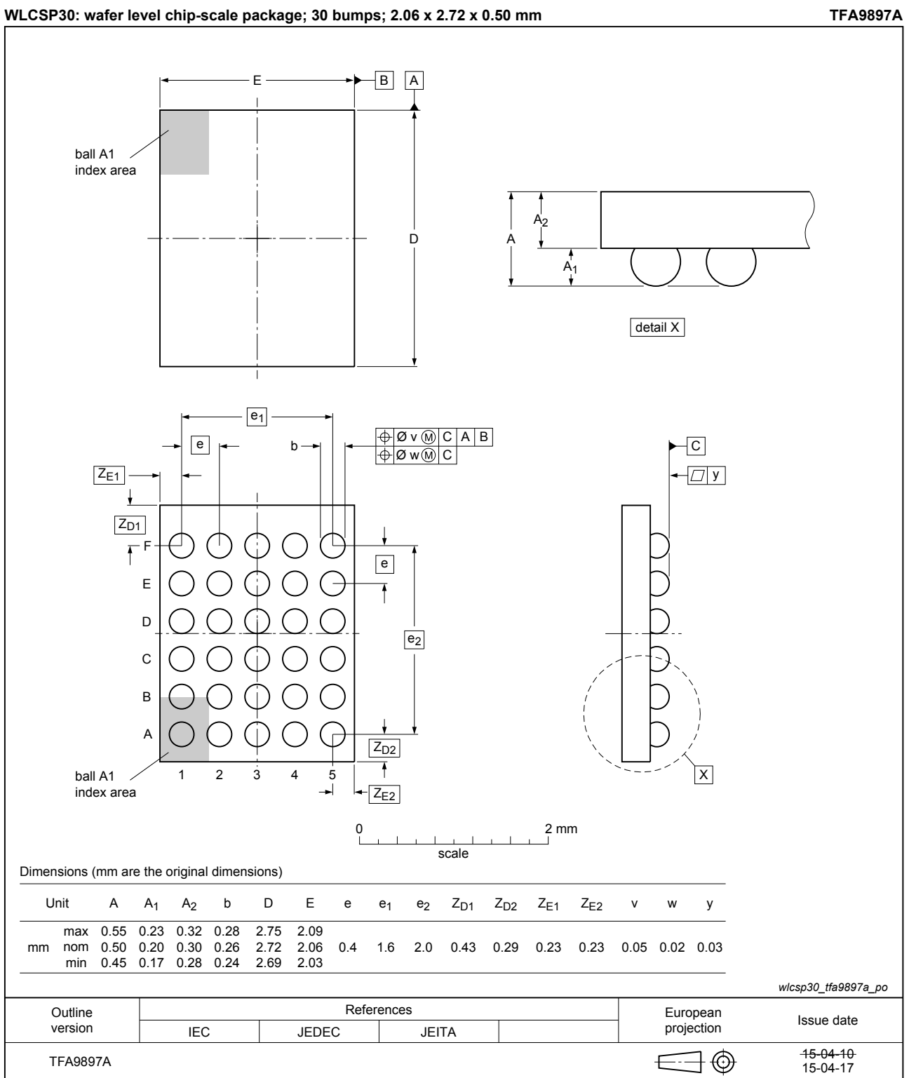
Fig. 1. Package outline WLCSP30 (OL-TFA9897A)
