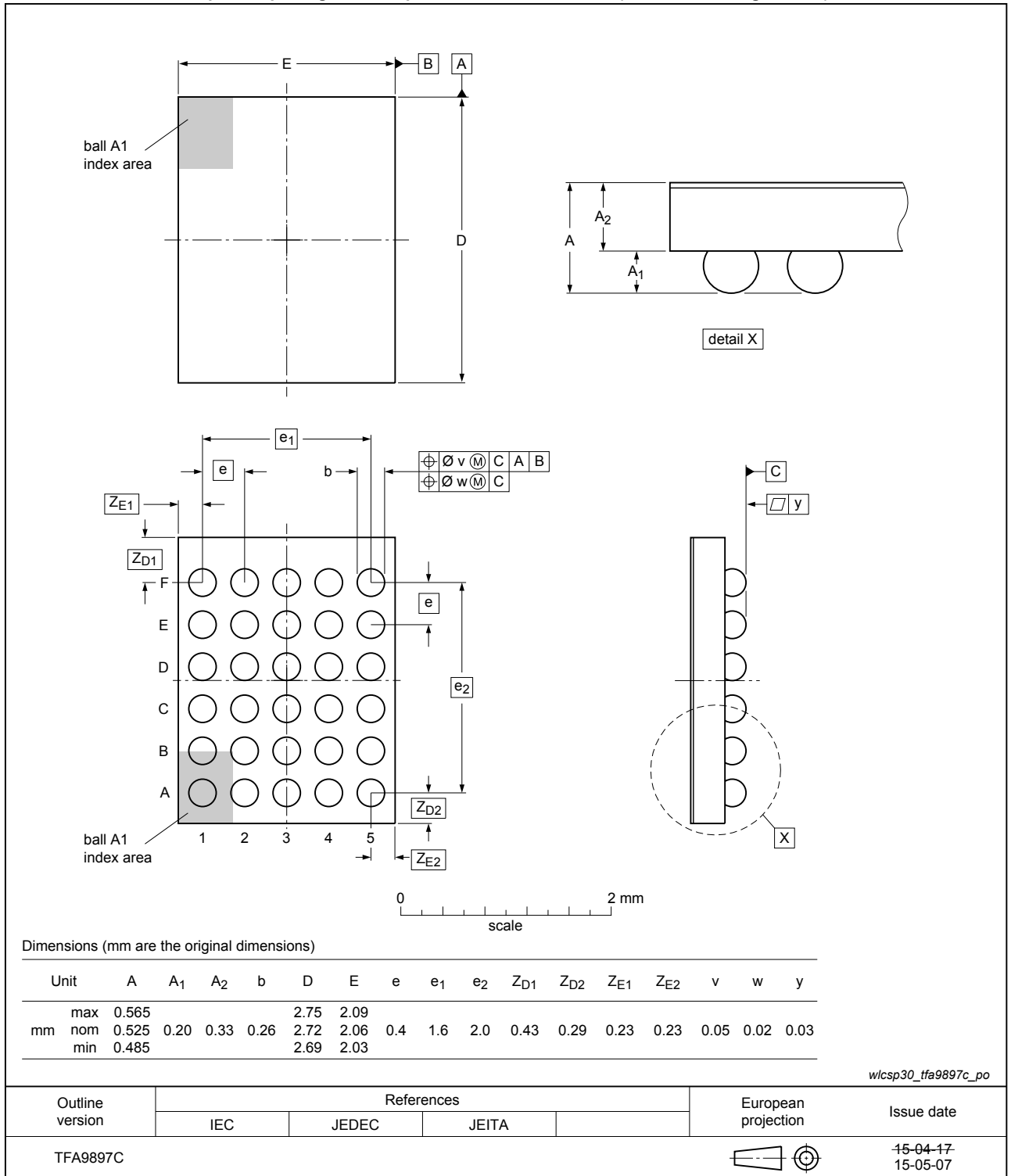
Fig. 1. Package outline WLCSP30 (OL-TFA9897C)
