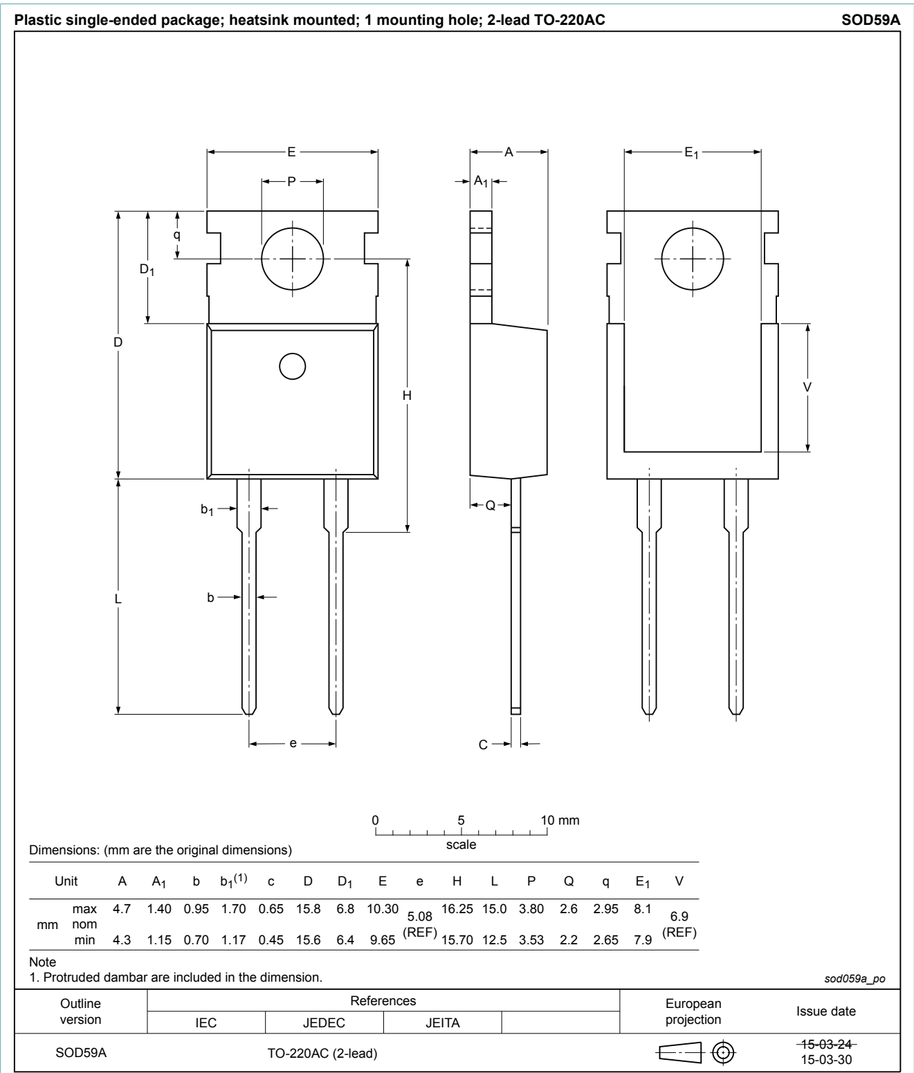
Fig. 1. Package outline TO-220AC (SOD59A)
