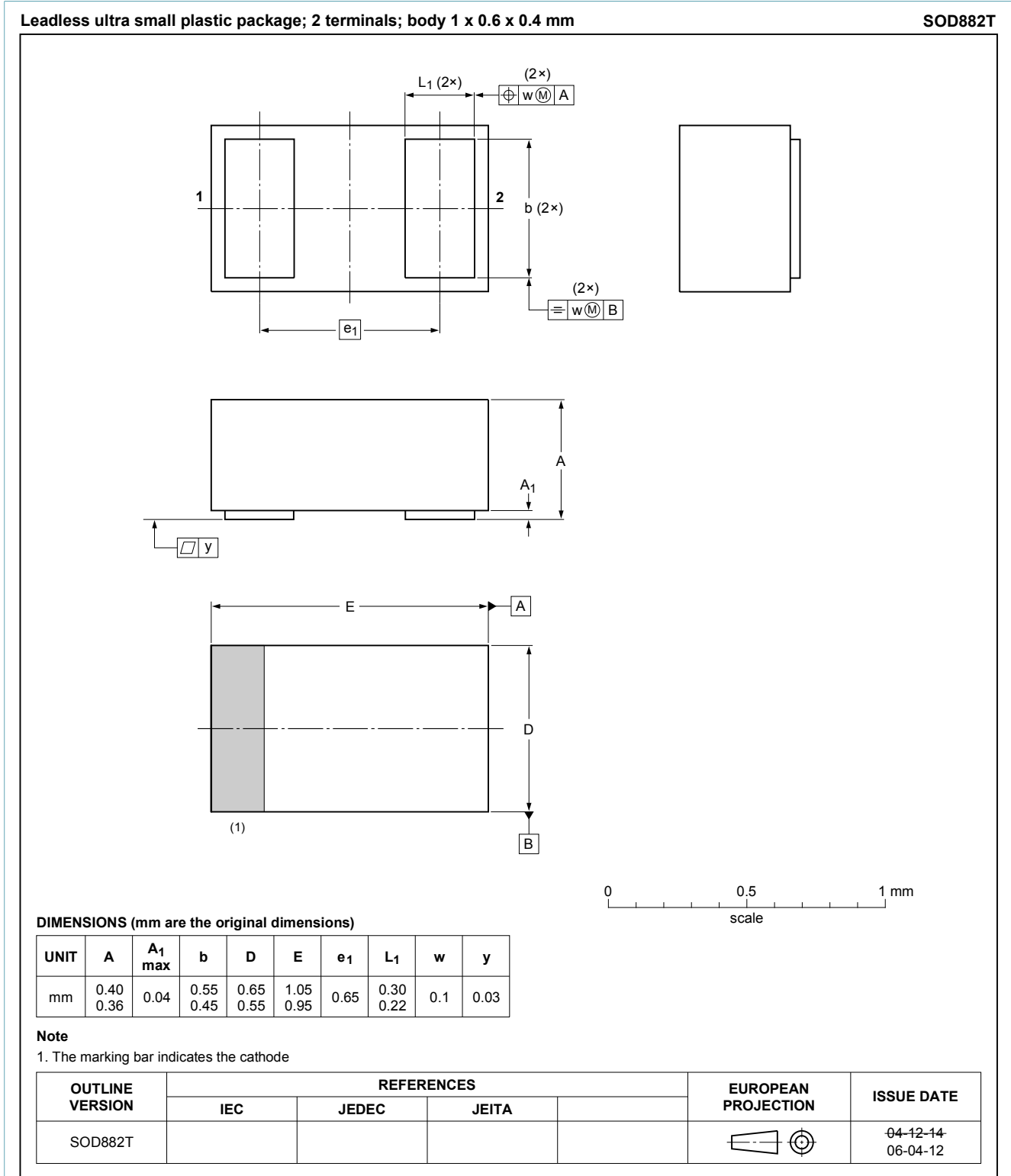
Fig. 1. Package outline SOD2 (SOD882T)
