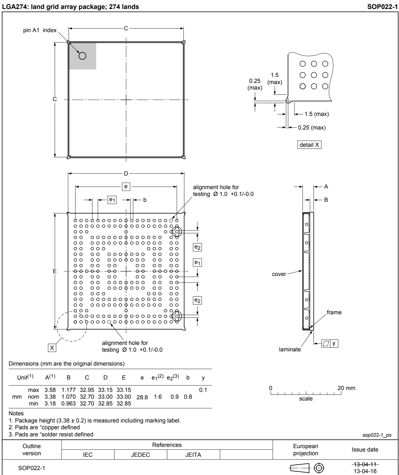
Fig. 1. Package outline LGA274 (SOP022-1)
