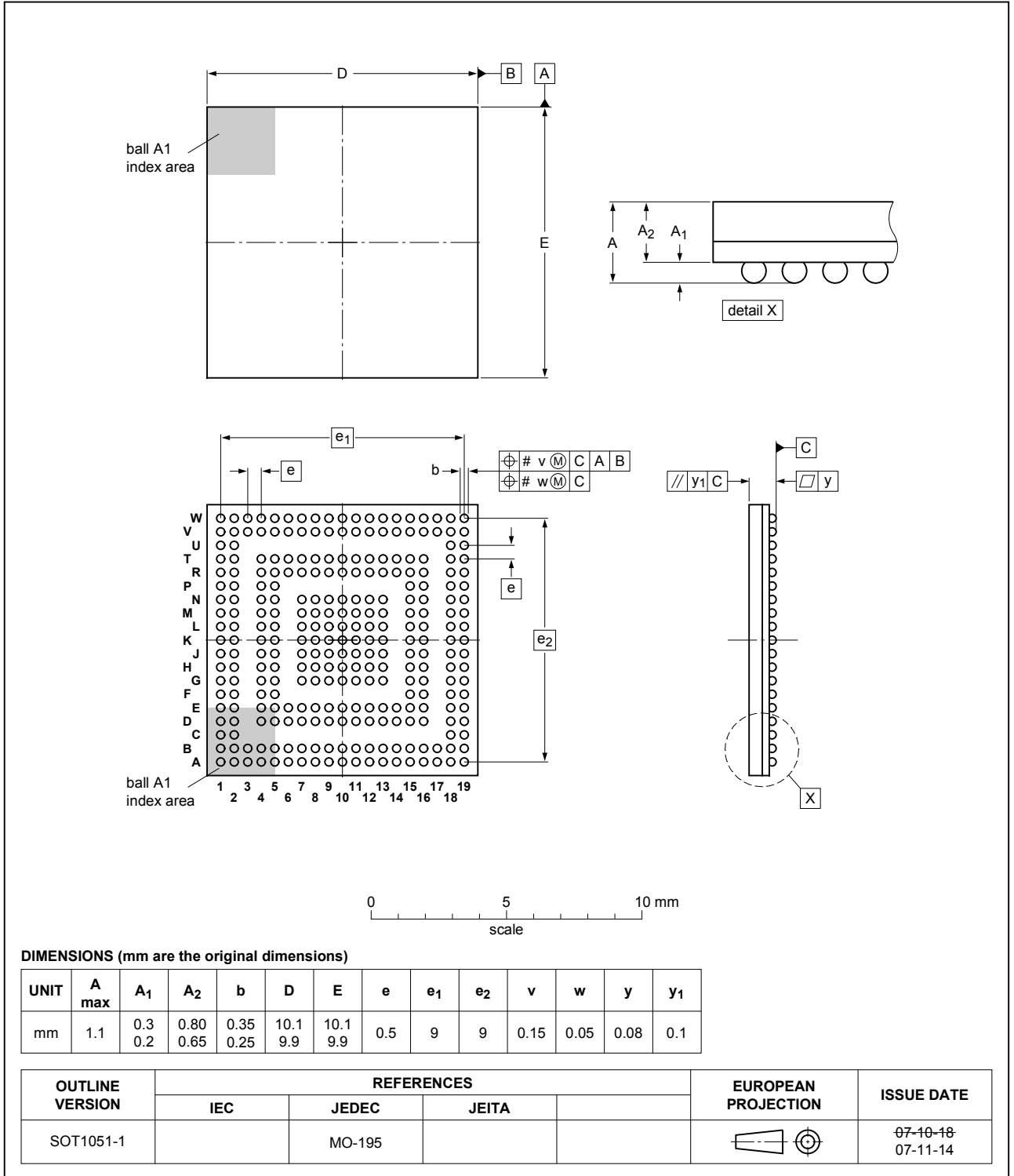
Fig. 1. Package outline TFBGA273 (SOT1051-1)
