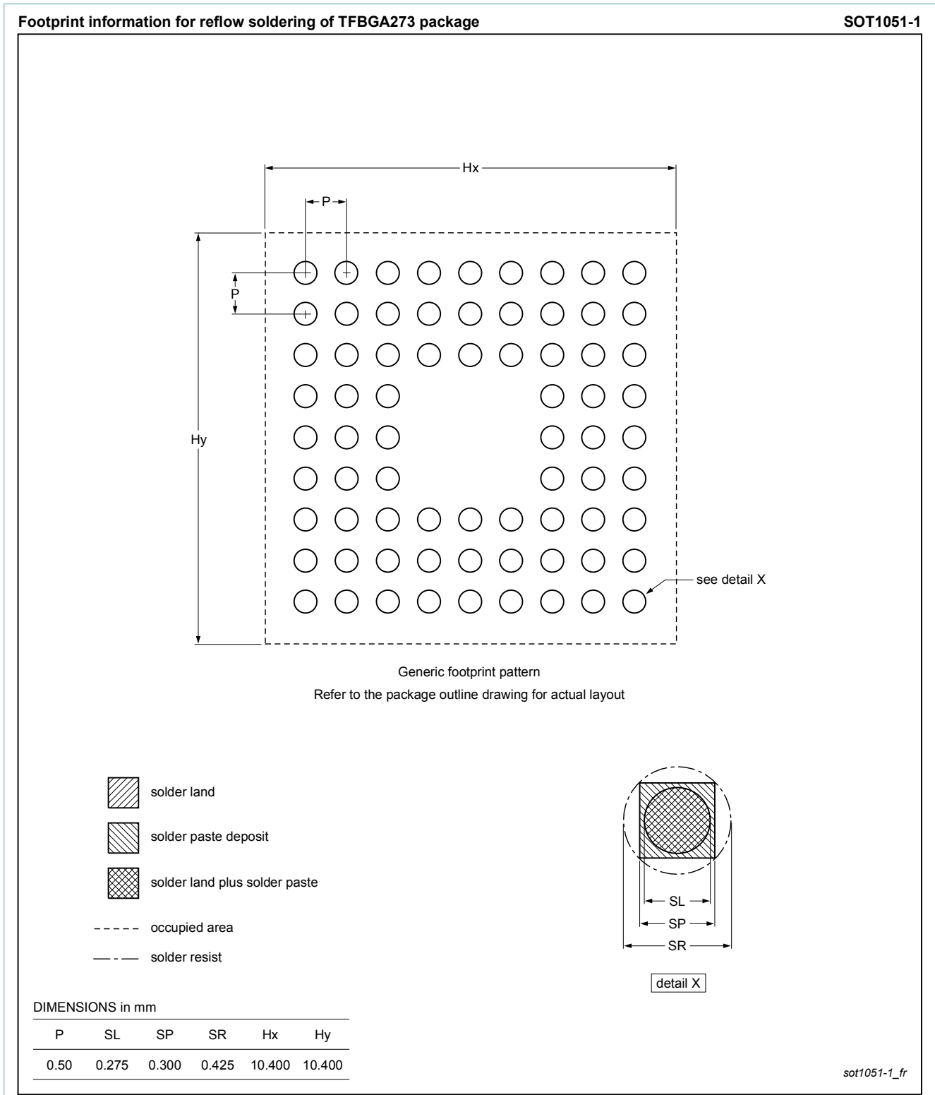
Fig. 2. Reflow soldering footprint for TFBGA273 (SOT1051-1)
