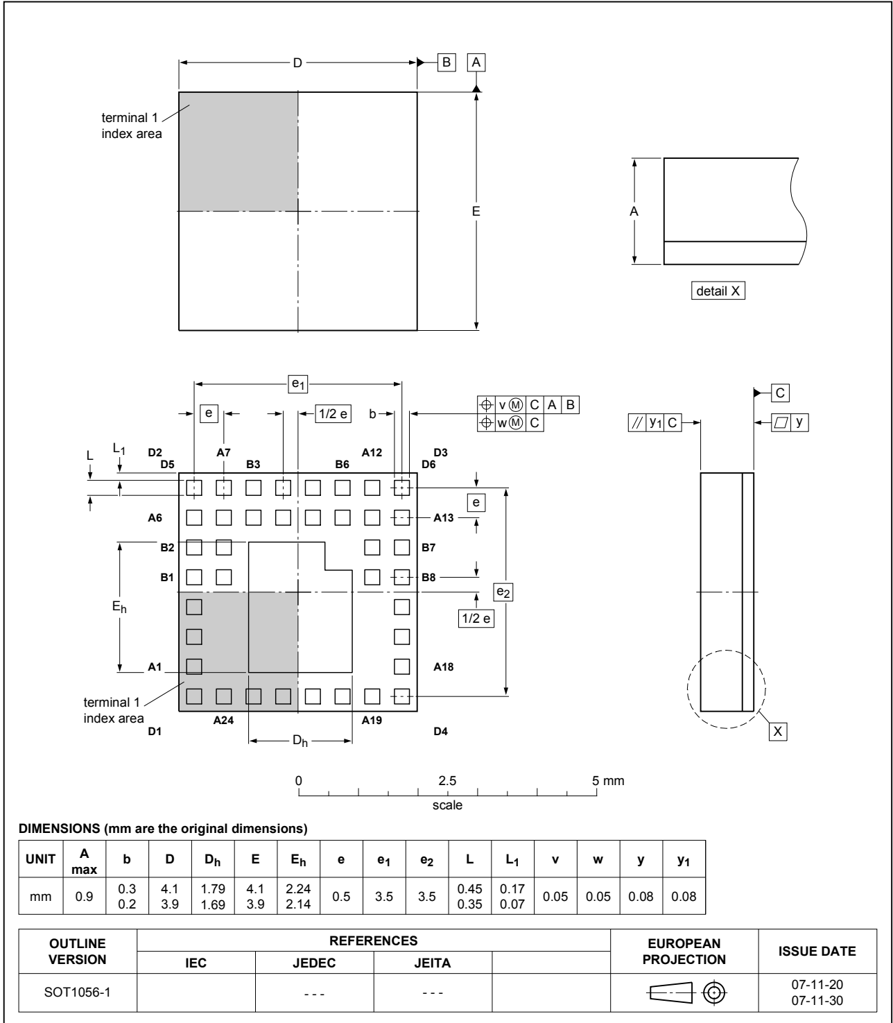
Fig. 1. Package outline HVQFN38R (SOT1056-1)
