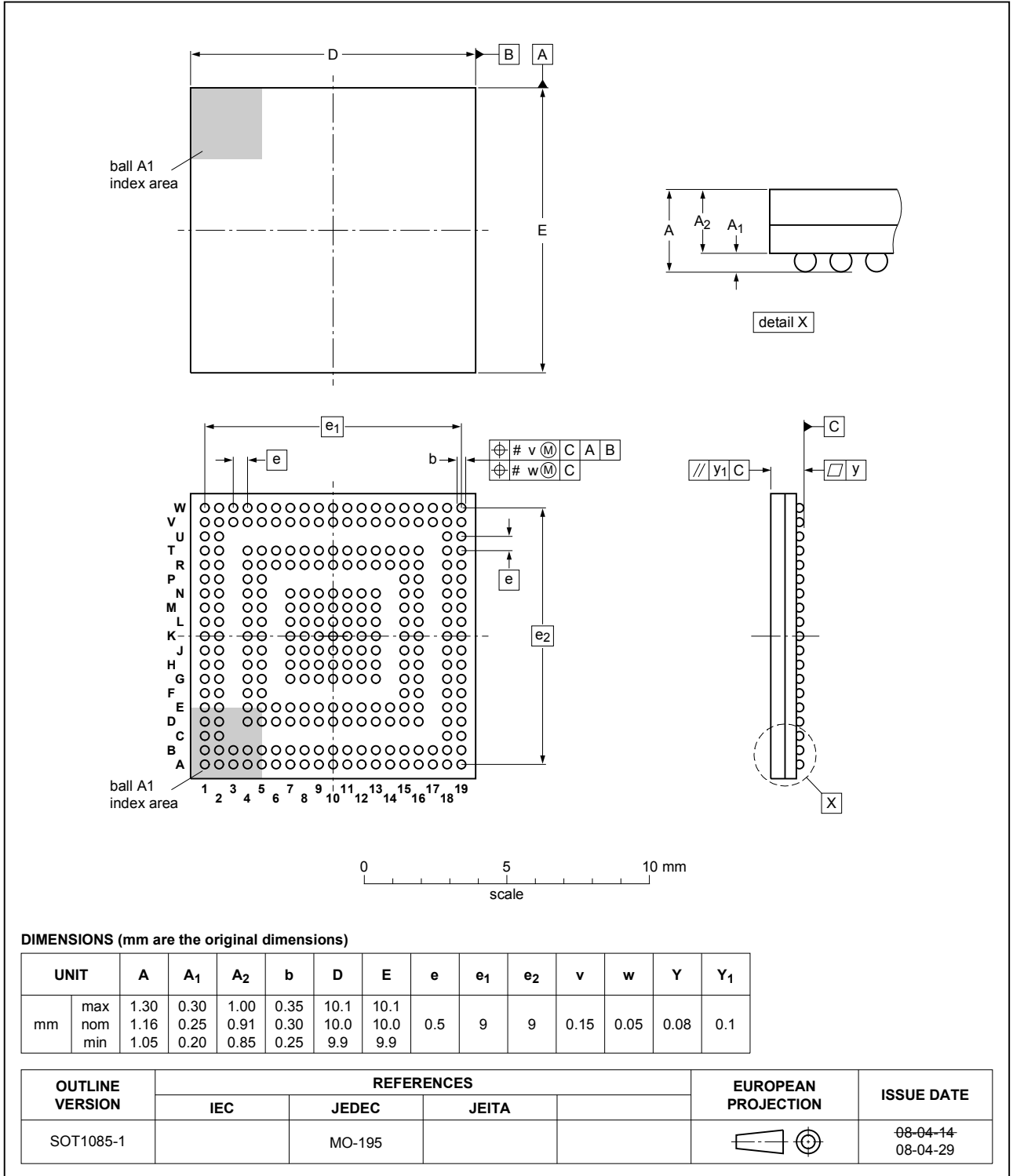
Fig. 1. Package outline LFBGA273 (SOT1085-1)
