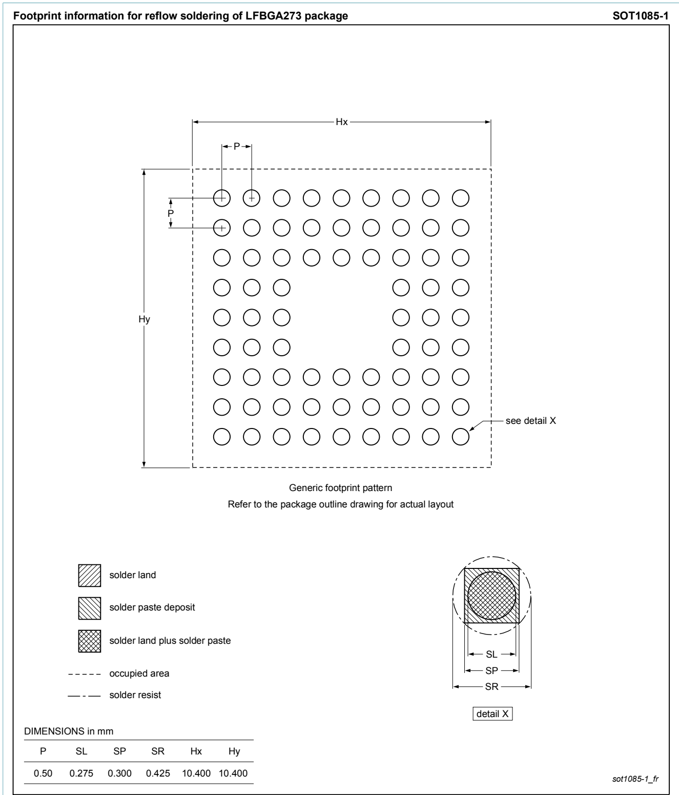
Fig. 2. Reflow soldering footprint for LFBGA273 (SOT1085-1)
