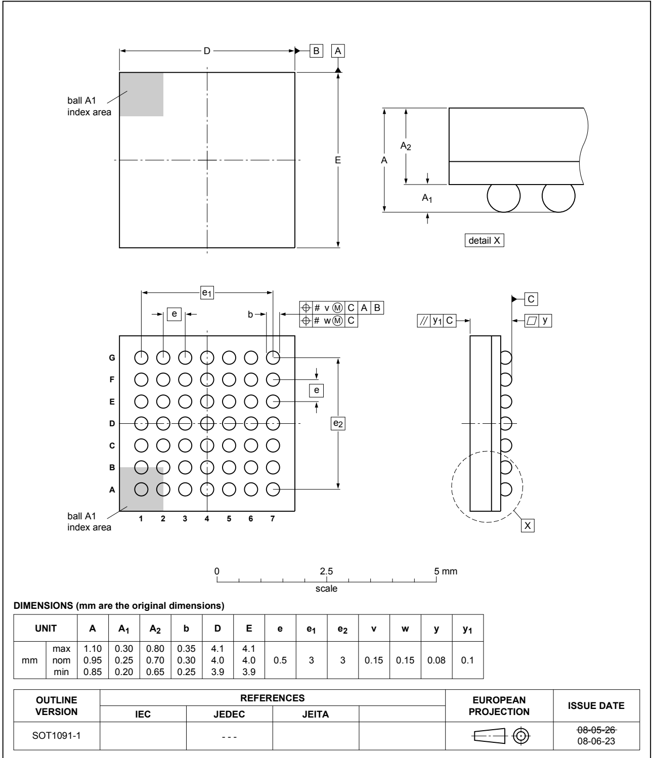
Fig. 1. Package outline TFBGA49 (SOT1091-1)
