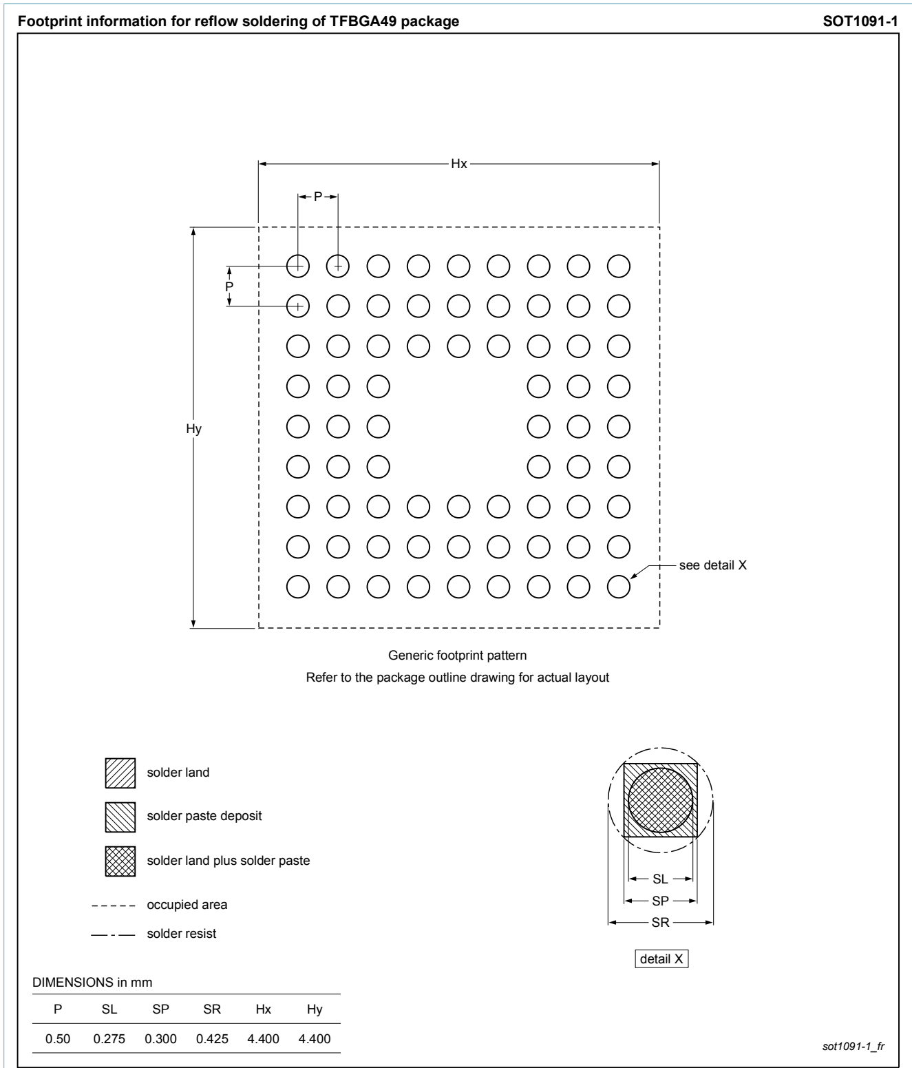
Fig. 2. Reflow soldering footprint for TFBGA49 (SOT1091-1)
