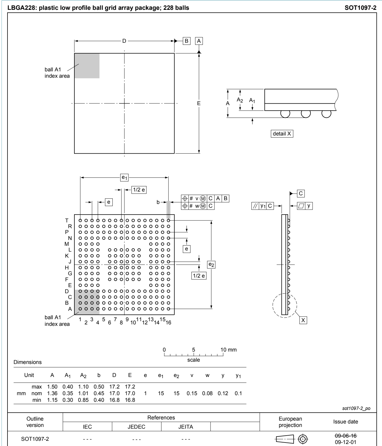
Fig. 1. Package outline LPGA228 (SOT1097-2)
