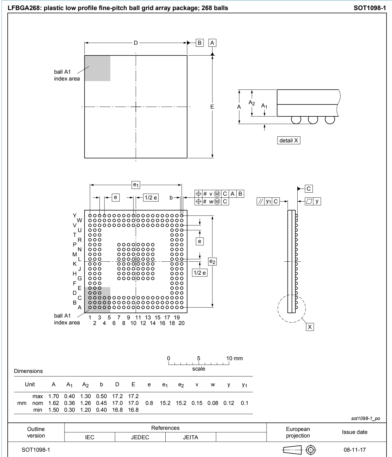
Fig. 1. Package outline LFPGA268 (SOT1098-1)
