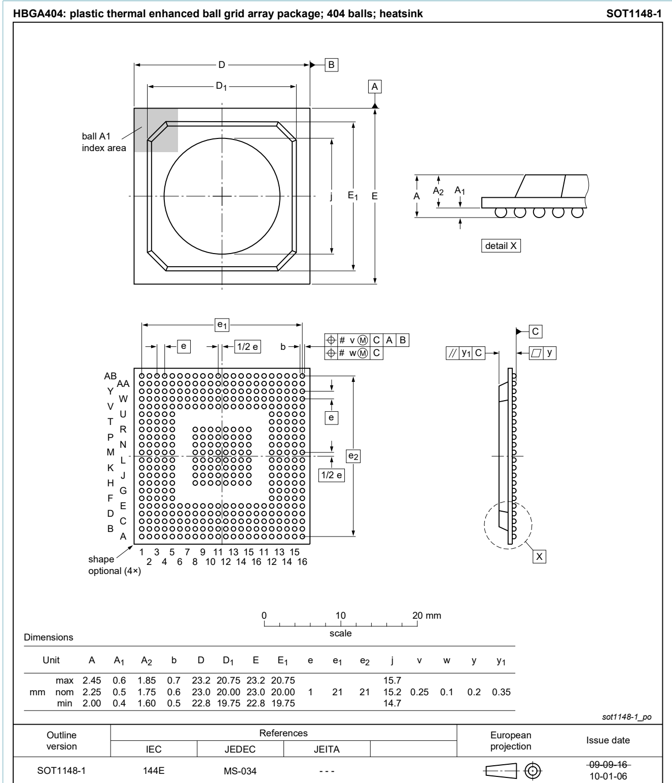
Fig. 1. Package outline HBGA404 (SOT1148-1)
