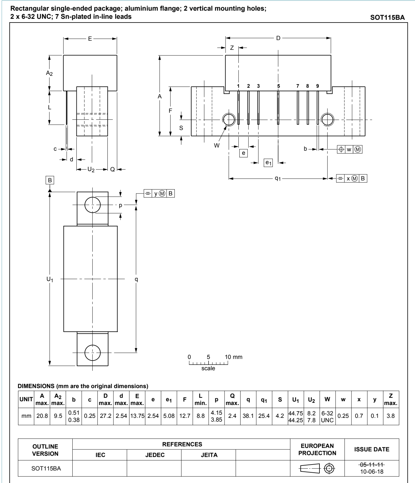
Fig. 1. Package outline SFM7 (SOT115BA)
