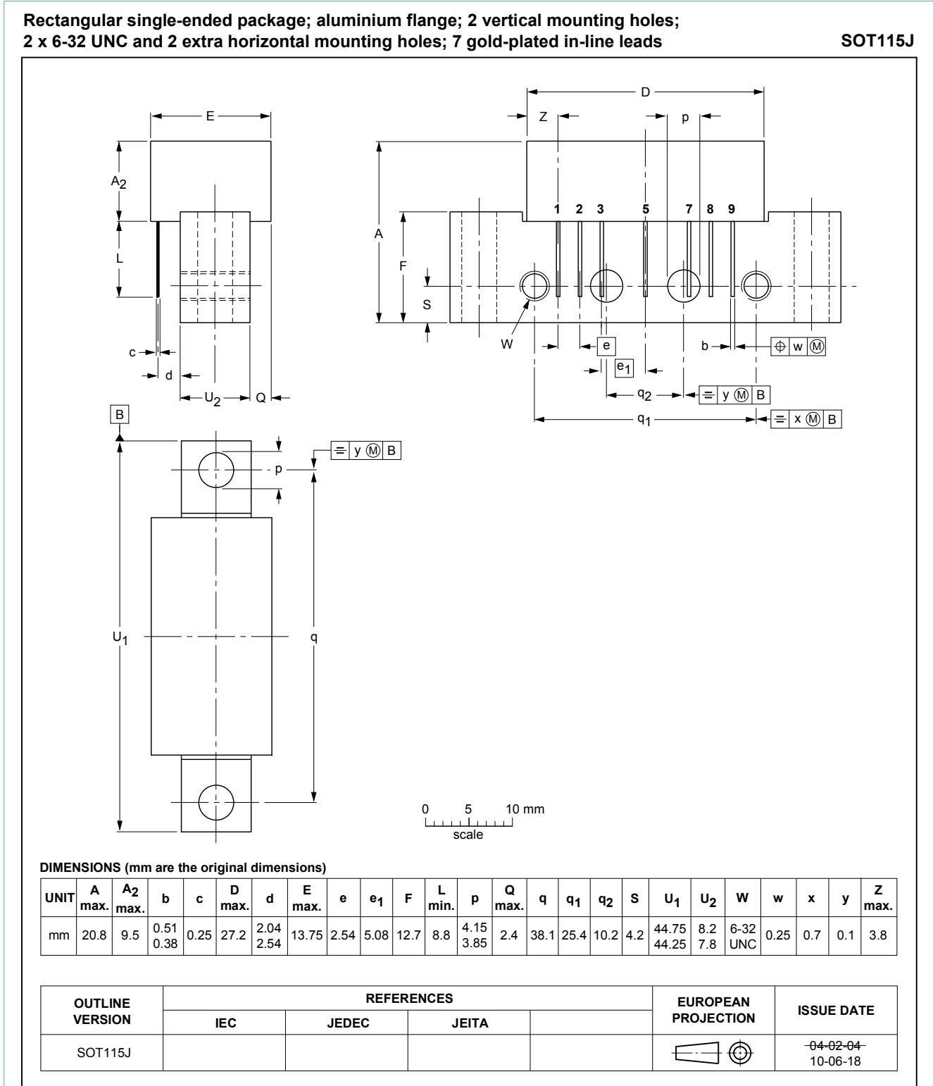
Fig. 1. Package outline SFM7 (SOT115J)
