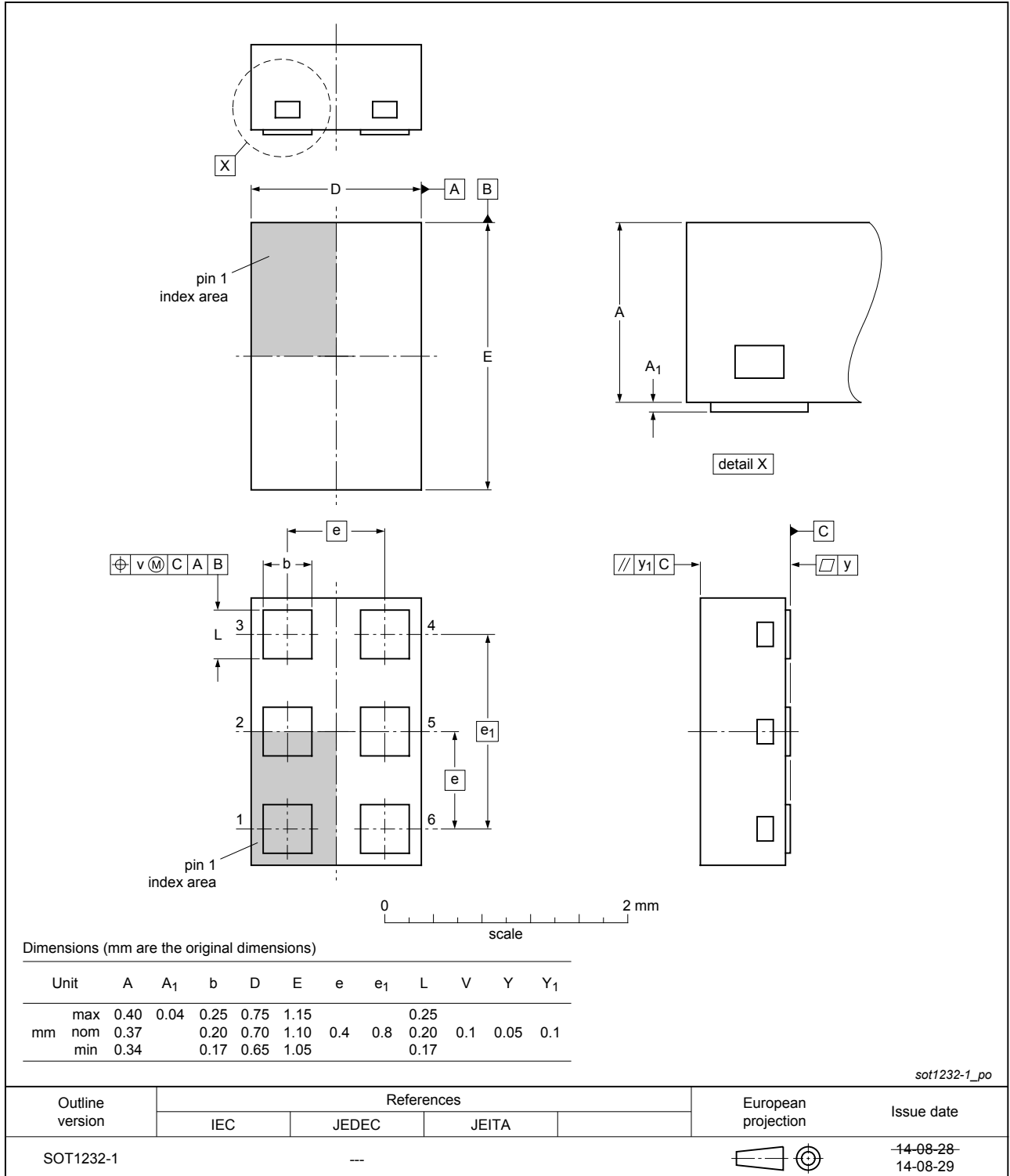
Fig. 1. Package outline FC-QFN6 (SOT1232-1)
