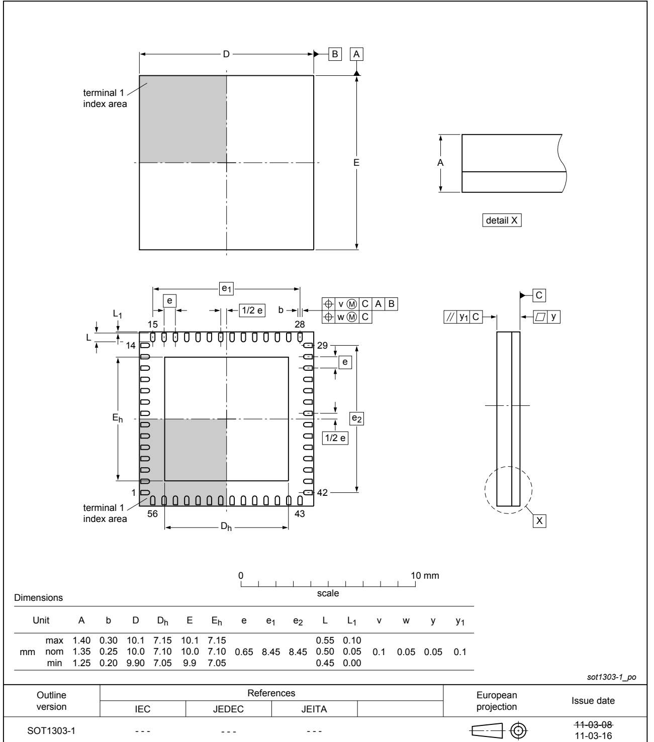
Fig. 1. Package outline HLQFN56R (SOT1303-1)
