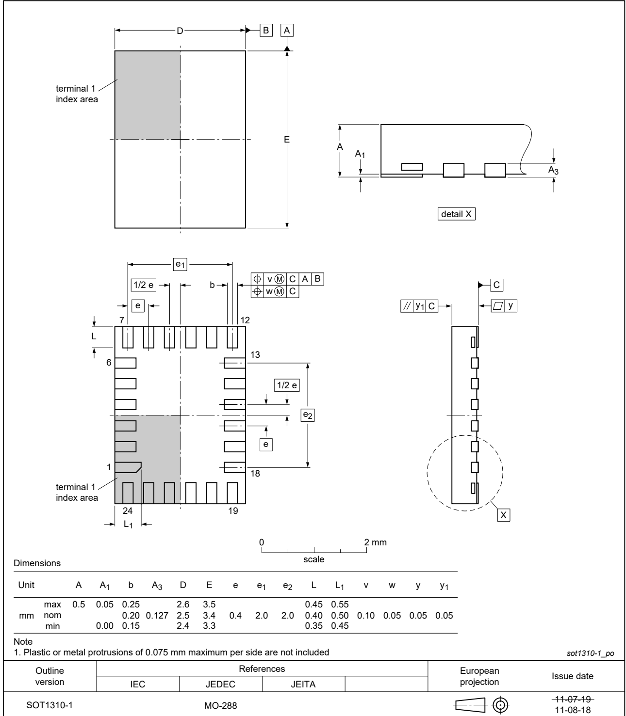
Fig. 1. Package outline XQFN24 (SOT1310-1)
