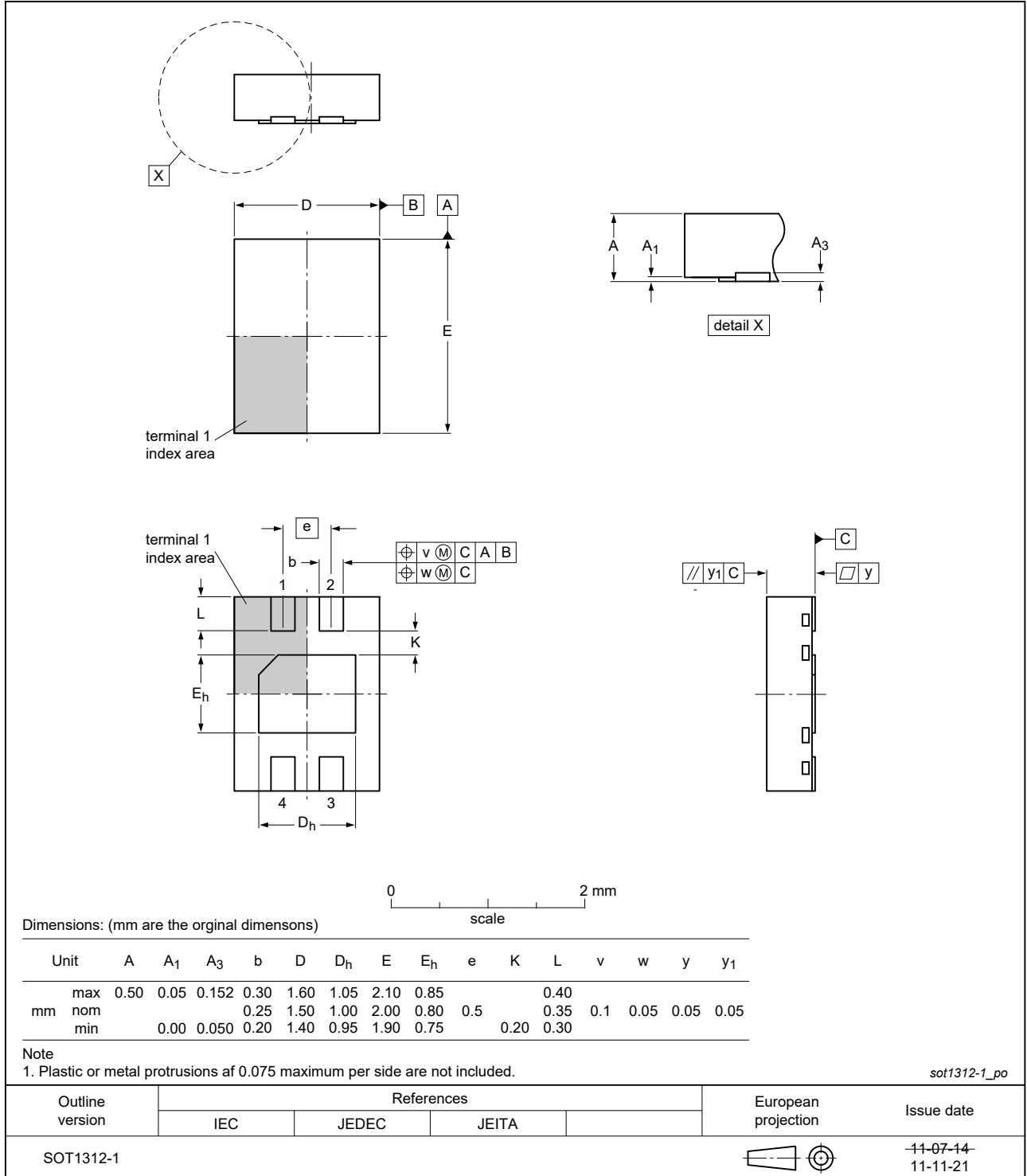
Fig. 1. Package outline HXSON4 (SOT1312-1)
