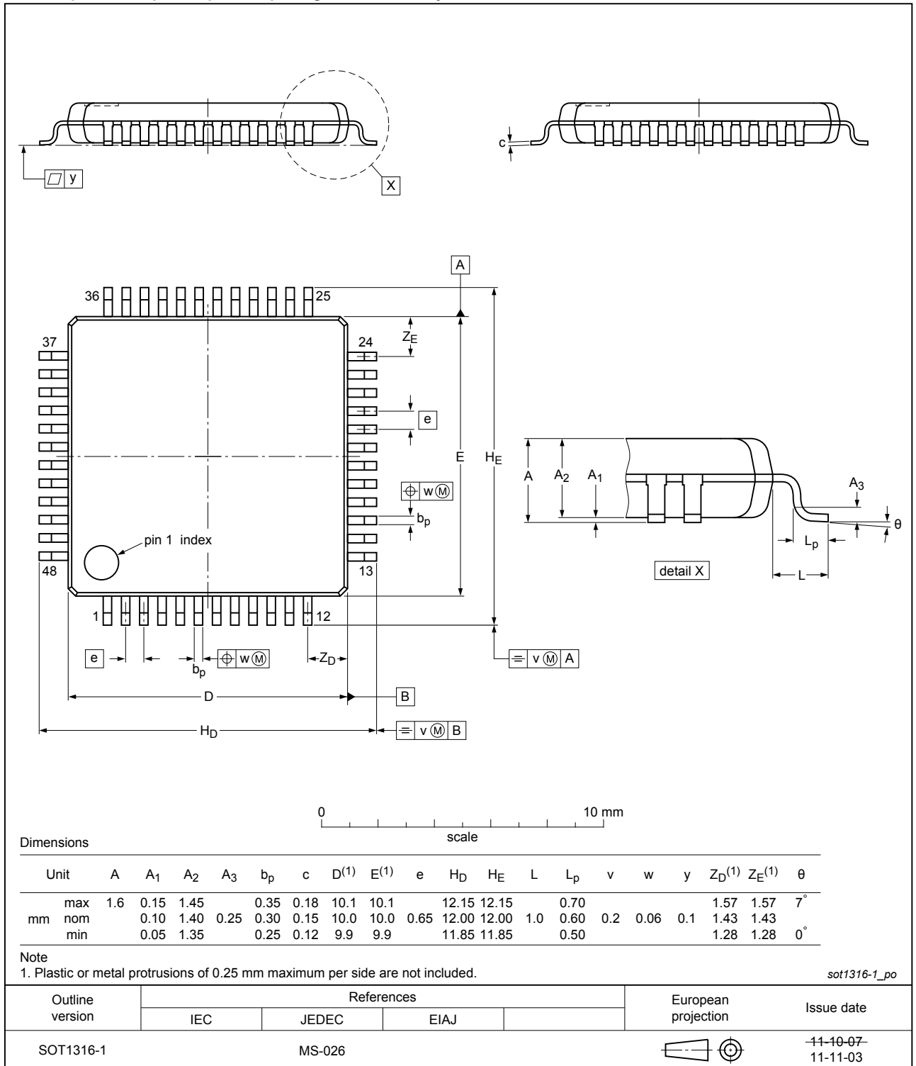
Fig. 1. Package outline LQFP48 (SOT1316-1)
