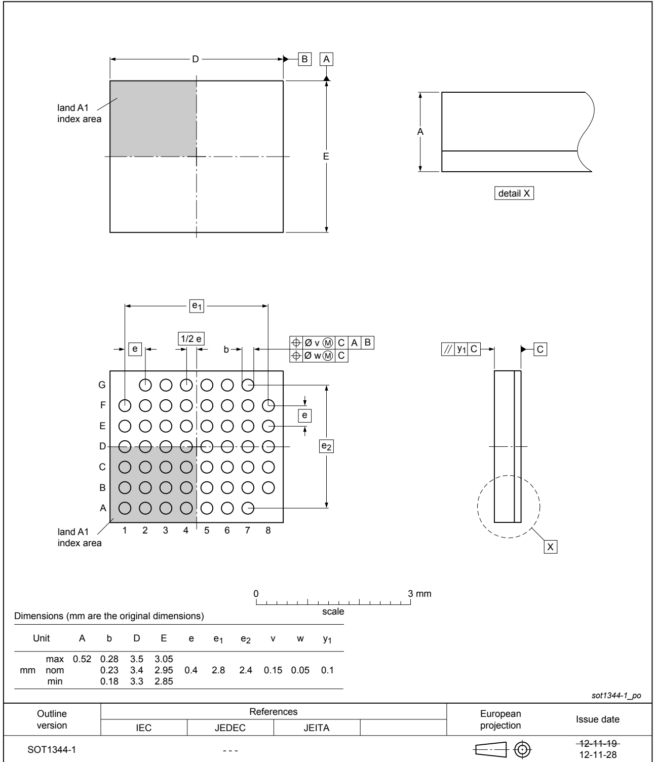
Fig. 1. Package outline UFLGA53R (SOT1344-1)
