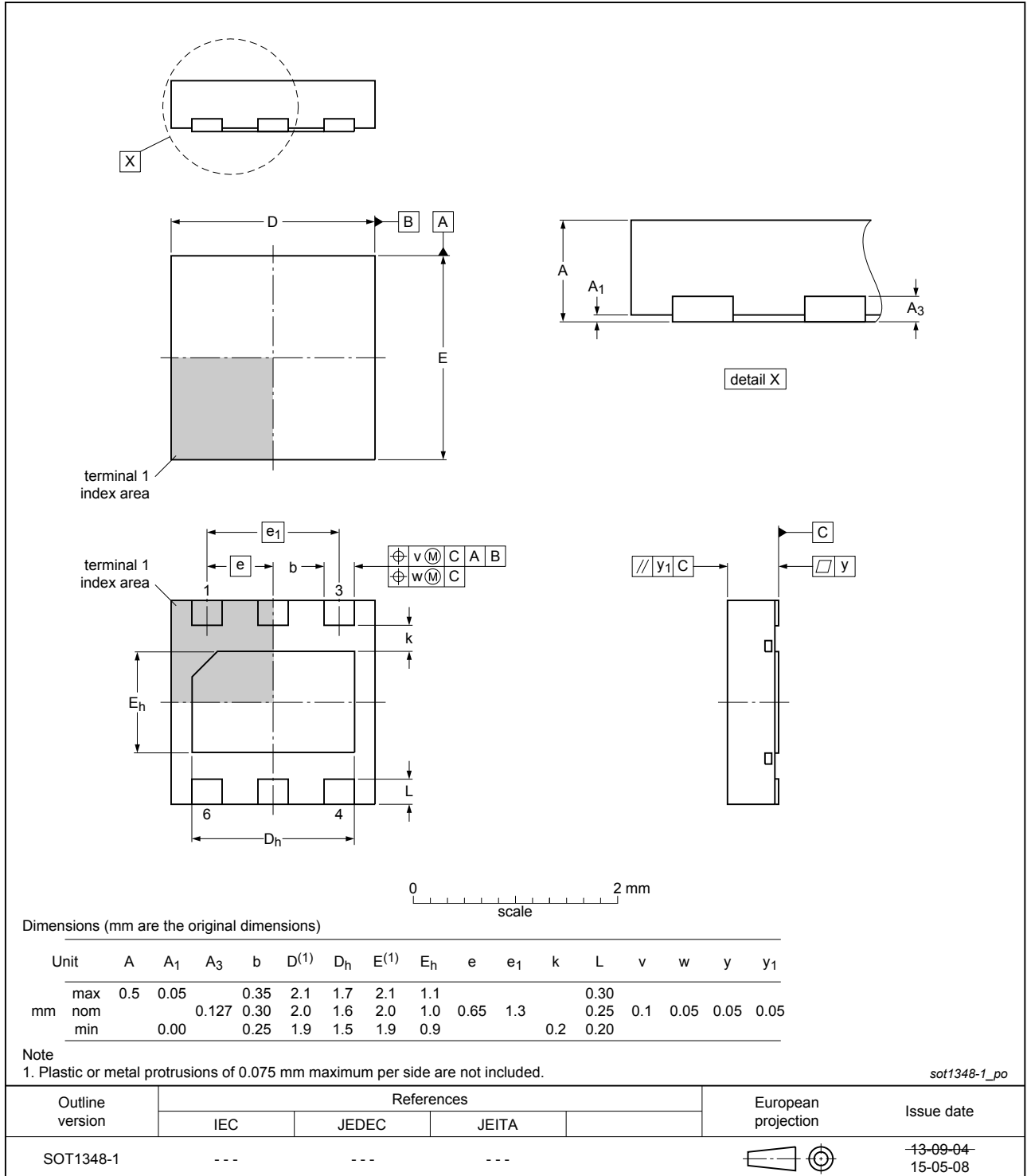
Fig. 1. Package outline HXSON6 (SOT1348-1)
